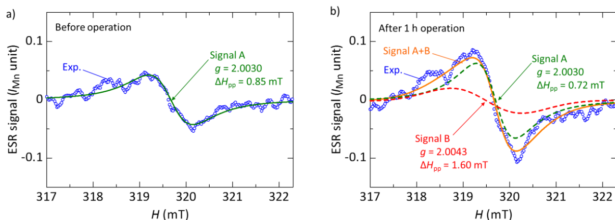
Figure 4. Fitting analyses of the ESR spectrum of the OLED before the device operation (a) and after 1 h device operation (b). The vertical axis is plotted using a unit of peak-to-peak ESR intensity of the ESR signal of a standard \text{Mn}^{2+} marker sample, I_{\text{Mn}} . a) The blue open circles show the experimental spectrum before the device operation. The green solid line shows the fitting result using a Lorentzian function. b) The blue open circles show the experimental spectrum after 1 h device operation. The green and red dotted lines show the fitting result using Lorentzian and Gaussian functions, respectively. The orange solid line shows the sum of these functions.
