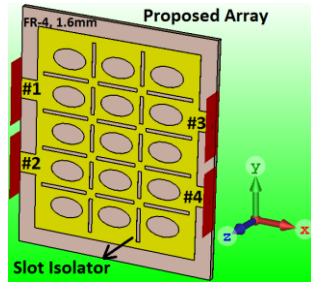
(b) Proposed waveguide slot array antenna
