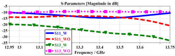
Fig. 2. S-parameters of the referenced and proposed waveguide slot array antennas without (WO) and with (W) linear slot isolators.
