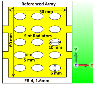
(a) Reference slot array antenna
