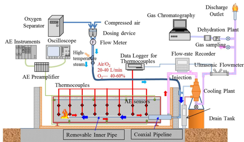
Figure 4. UCG experimental system, the coaxial-hole model.
