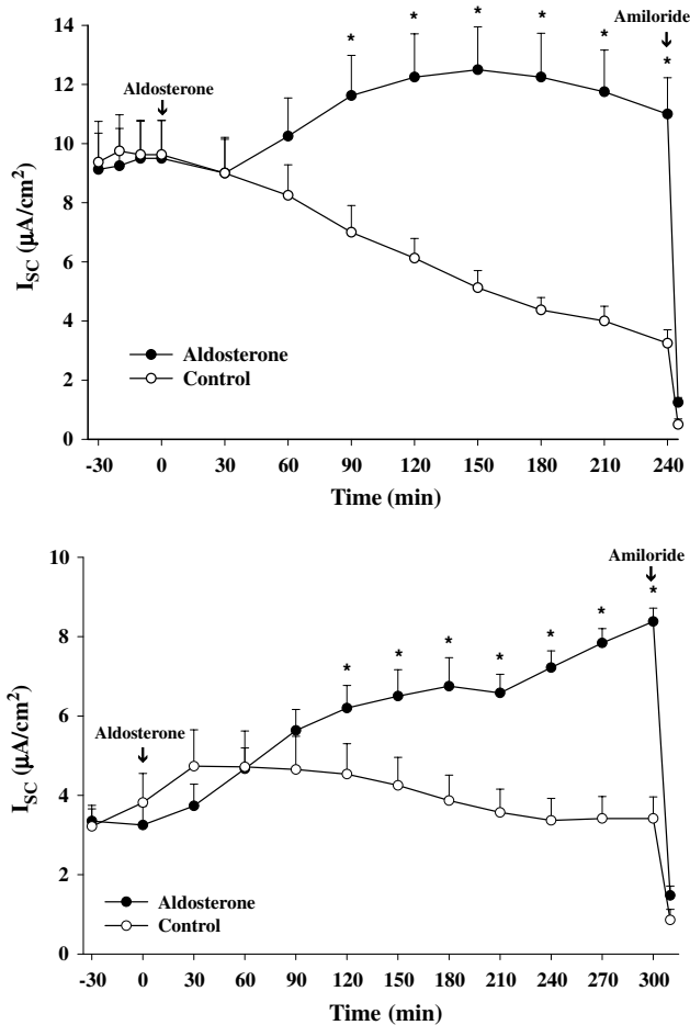
Fig. 1. Aldosterone-induced Na^+ I_{SC} in renal principal cells. In each series of experiments, a maximal dose of aldosterone ( 2.7 \mu M ) was added at time = 0 \text{ min} to the serosal bathing media of monolayers formed by either the mpkCCD c14 (upper panel) or A6 cell line (lower panel). Amiloride ( 10 \mu M ) was added apically at the end of each experiment. Symbols represent the mean of n experiments \pm SEM. As determined by Student's t test, aldosterone caused a significant increase in reabsorptive Na^+ flux beginning at 90 and 120 min post-hormone addition in mpkCCD c14 ( n = 8 ) and A6 ( n = 6 ) cells, respectively. *p \leq 0.05 .
