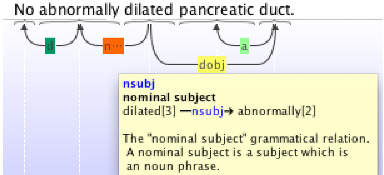
Fig. 4. Dependency relation for a sentence with “ nsubj ” relation
