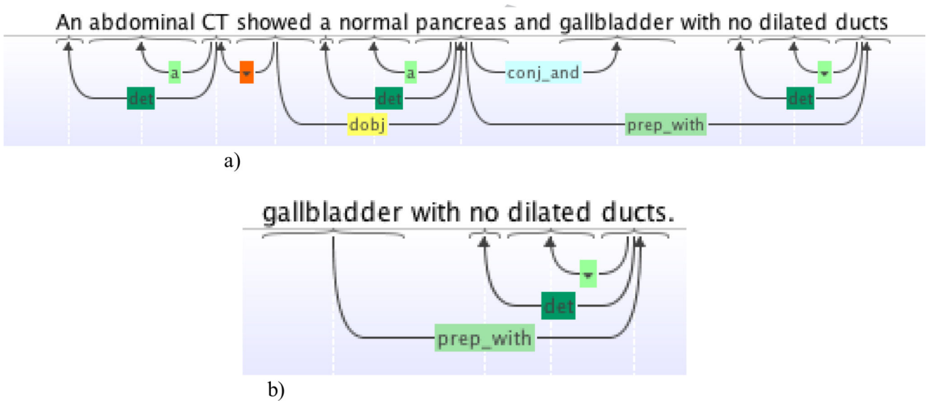
Fig. 3. a) Dependency relation for a sentence with “prep_with” relation b) SDP after splitting the sentence into two sentences
