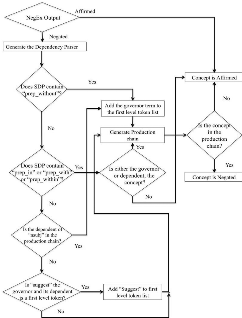
Fig. 1. Detailed flowchart of the DEEPEN algorithm
