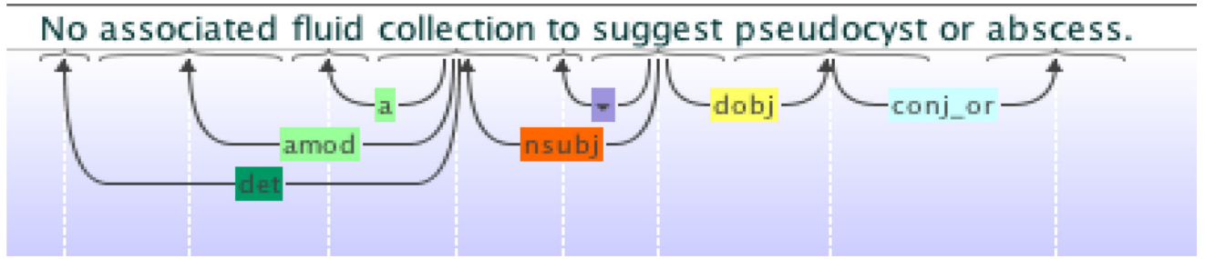
Fig. 5. Dependency relation for a sentence with “suggest” as the dependent term
