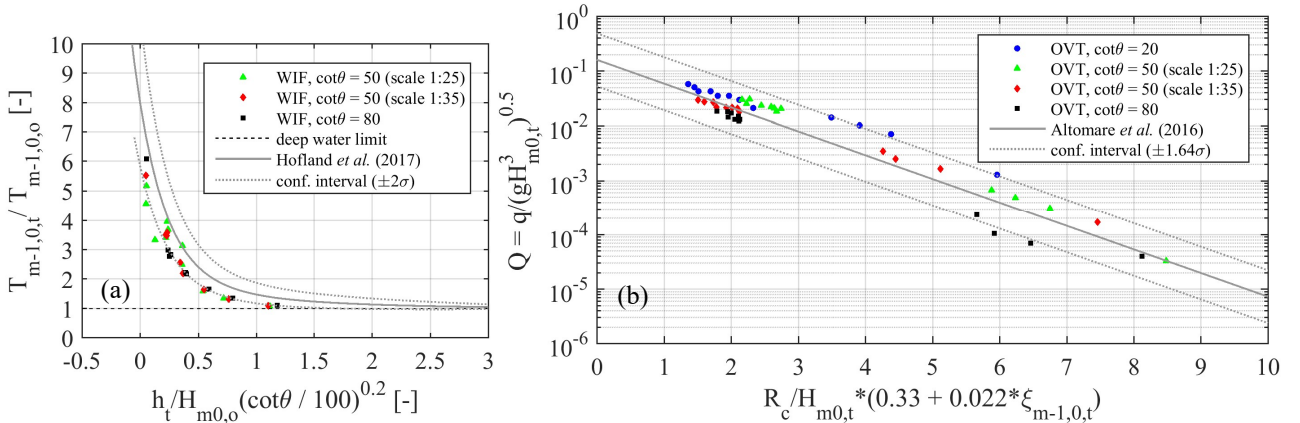
Figure 5. (a) Dimensionless spectral wave period at the toe of the dike versus the relative water depth with slope correction. Experimental data compared to Equation 2 for the test results in the small channel during the wave impact force (WIF) experiments with second order wave generation. The WIF small channel results were chosen to be plotted here, because the correspondence with the IWC tests was best. (b) Semi-logarithmic plot (x-axis: linear scale, y-axis: logarithmic scale) of the dimensionless wave overtopping Q in function of the dimensionless freeboard with shallow foreshore correction and equivalent slope. The experimental wave overtopping results (OVT) of the tests with second order wave generation for all foreshore slopes is compared to the prediction formula of Altomare et al. (2016) with the equivalent slope concept.
