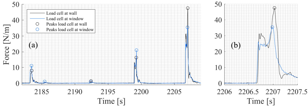
Figure 6. Comparison of the two load cell measurements, spaced 0.20 m from each other along the vertical wall on top of the dike. Impacts are shown for RS06, slope 1/50 at scale 1:25. (a) Overview of some impacts, (b) zoom to maximum force peak.
