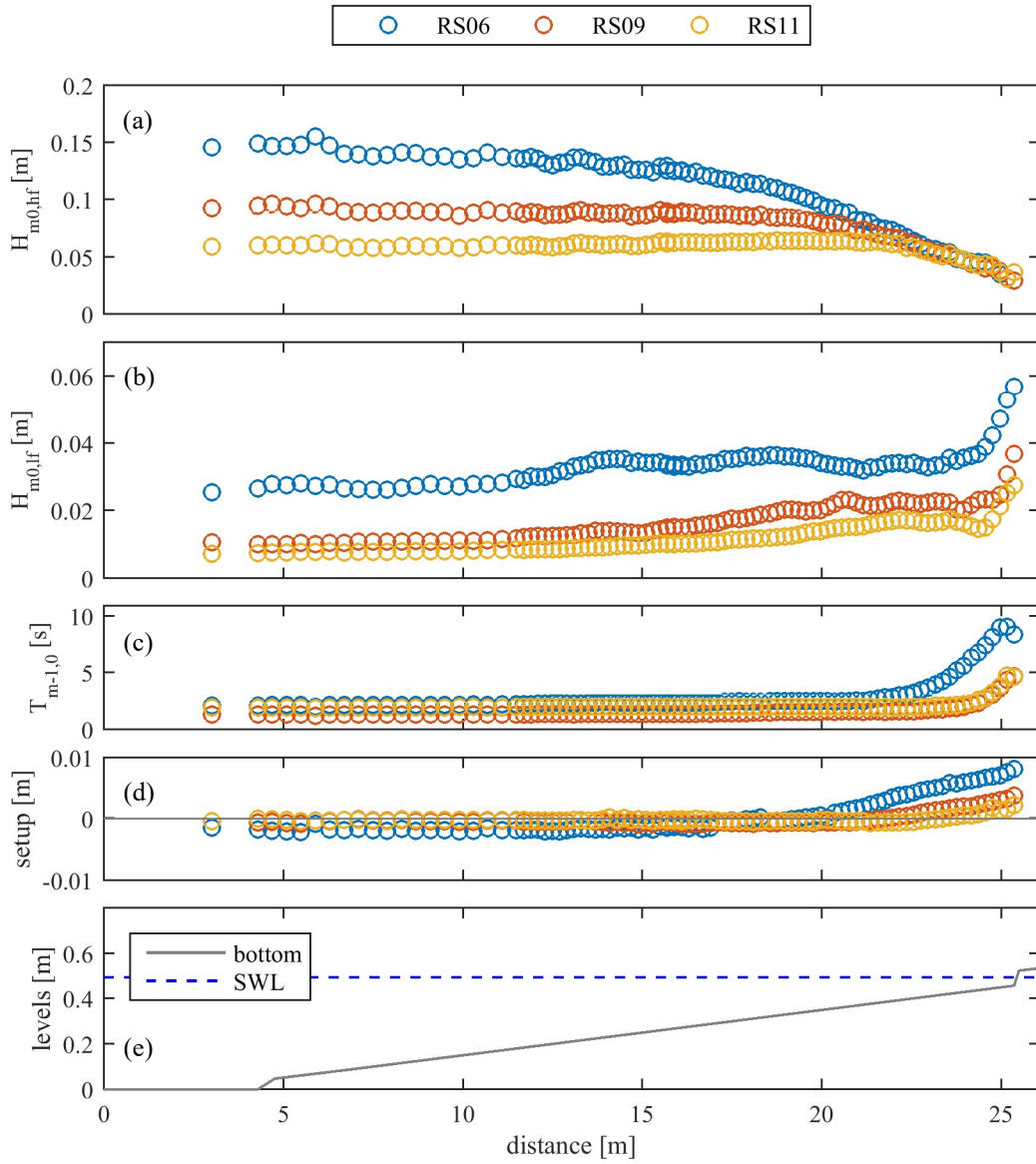
Figure 3. The wave characteristics measured over the complete foreshore (slope 1/50), by way of repeated and combined HSR experiments at model scale 1:35, (a) the short wave (hf: high frequency) significant wave height H_{m0,hf} , (b) the infragravity wave (lf: low frequency) significant wave height H_{m0,lf} , (c) the spectral wave period T_{m-1,0} , (d) the wave setup and (e) the bottom profile with indication of the still water level (SWL).
