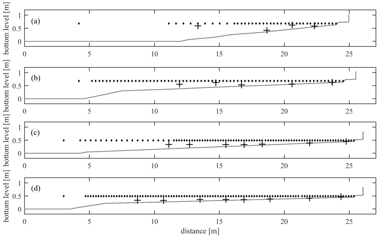
Figure 1. Tested cross-shore bottom profiles, consisting of a dike geometry with foreshore slopes: (a) 1/20 (model scale 1:25), (b) 1/50 (scale 1:25), (c) 1/50 (scale 1:35), (d) 1/80 (scale 1:35). Bed level z (flume bottom at z = 0.0 m) is shown by the grey line over the cross-shore distance x from the wave-maker zero position ( x = 0.0 m). The diamond shaped points are the wave gauge positions plotted at the highest water level tested and the pluses are the positions and heights of the electromagnetic current meter for the high spatial resolution tests.
