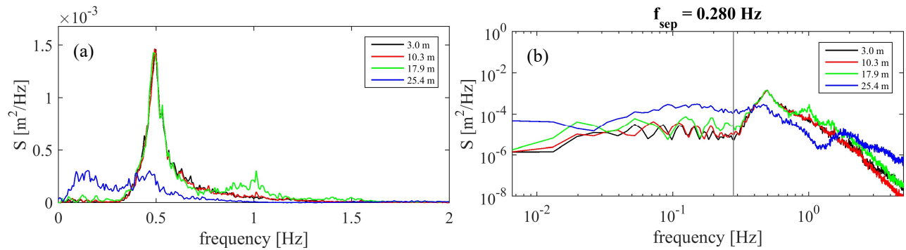
Figure 4. Spectral variance density S over frequency f of condition RS11 at four equidistant locations along the flume (foreshore 1/50 at model scale 1:35, see Figure 1b and Figure 3), starting at the reference wave gauge and ending at the wave gauge at the toe of the dike, (a) linear scale axes, (b) logarithmic scale axes, with indication of the separation frequency f_{sep} (gray line).
