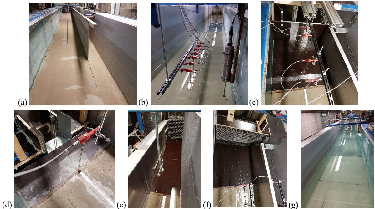
Figure 2. Model set-up pictures: (a) view on the 1/50 foreshore slope and separation wall towards the dike, (b) first array of 7 wave gauges and one co-located ECM for the high spatial resolution tests, (c) model set-up for wave impact measurements, (d) wave overtopping set-up, (e) view on the small separated channel with absorption material, (f) model set-up for the incident wave conditions at the toe of the dike, and (g) view towards the end of the 1/20 foreshore slope.
