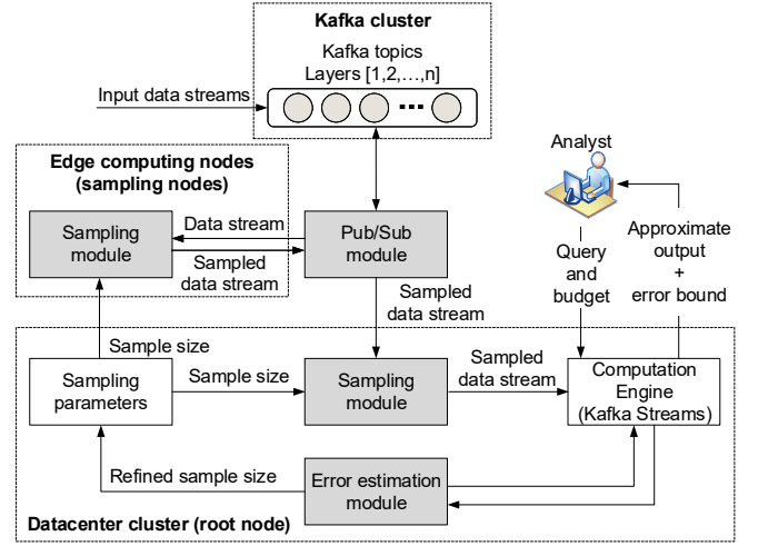
Fig. 4. APPROXIOT architecture.
