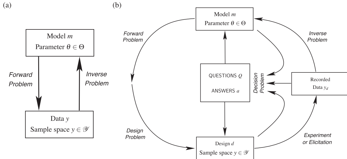
Figure 1 (a) Classical schema for solving inverse problems: the data y are assumed to come from a model m , parametrized by \theta . The inverse problem is the estimation of the set of parameter values \theta that will generate data in the forward problem that best match the observed data. (b) Schema for ‘interrogation problems’: given a set of scientific questions Q and a model m or range of models (Sambridge et al. 2006), an experimental design is selected to generate data y_d that best constrain the model parameters \theta and thereby answer the questions. Feedback occurs through the modification of the questions in the light of the answers, and the process can repeat. This schema is embodied algorithmically in Fig. 2.
