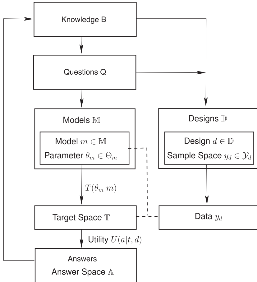
Figure 2 Algorithmic schema of an interrogation problem. See the text for details.
