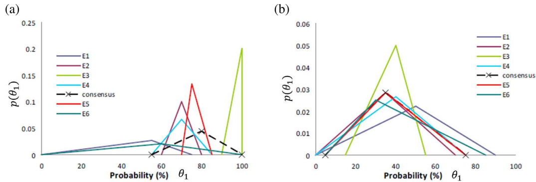
Figure 5 Individual and consensus probability distributions for p(\theta_1) elicited from six experts (E1–E6) under designs (a) d_1 and (b) d_2 discussed in the text. From a study similar to that of Polson & Curtis (2010, 2015).
