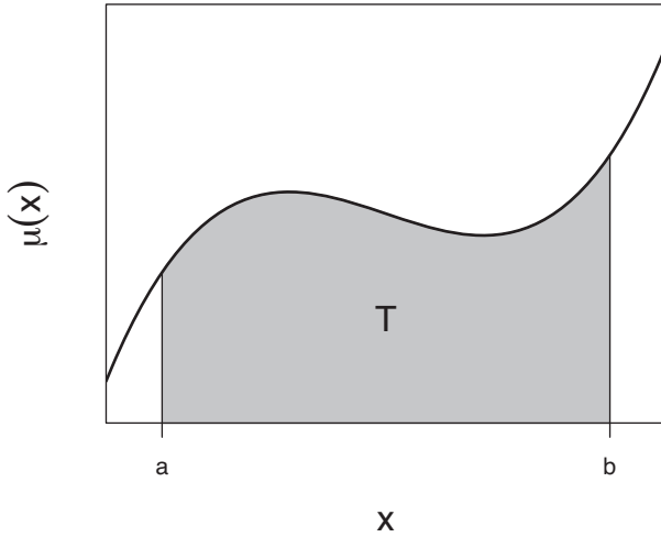
Figure 3 Example integral T = \int_a^b \mu(x)dx giving the shaded area under the graph. The investigator wants to estimate the value of T , with the precise form of \mu(x) being only of secondary interest.
