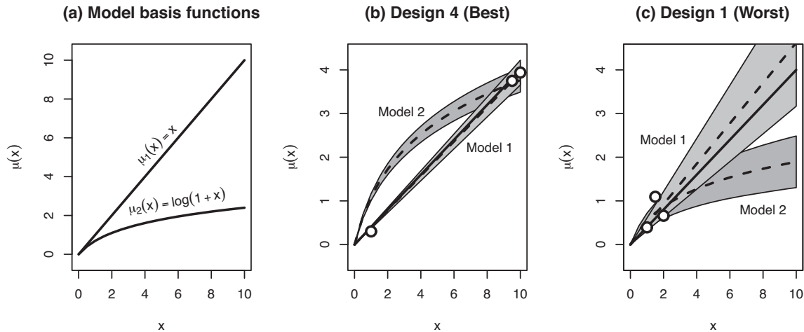
Figure 4 (a) Basis functions for the two models; (b) and (c) show the best fits for Models 1 and 2 under the best ( d_4 ) and worst ( d_1 ) of the five designs, given the data simulated under Model 1 with \theta = 0.4 (Table 3). The true model is shown as a solid line, the simulated data are shown as open circles. The shaded areas around the fitted curves are the 95 per cent posterior credible intervals for the fitted models.
