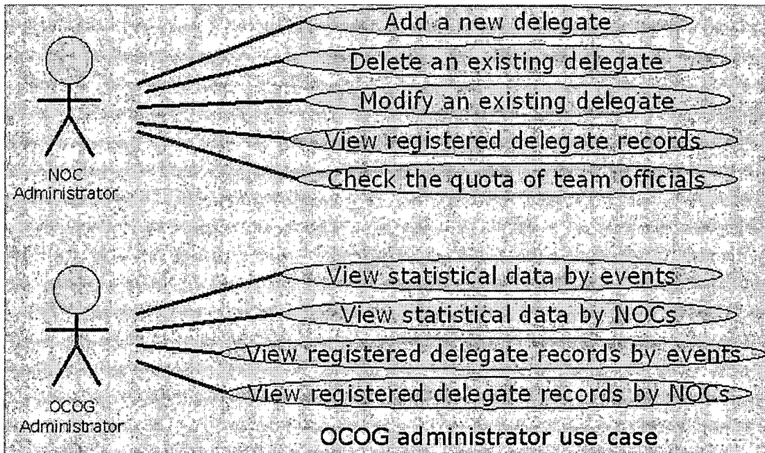
Figure 4. User Case Diagram
