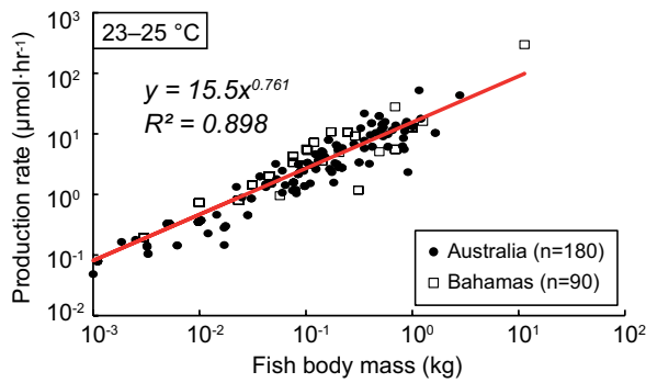
Figure 3. CaCO 3 production rate–body mass relationship at 23–25 °C, based on data from Australia (this study) and the Caribbean (Perry et al., 2011).
