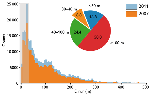
Fig. 4. Histograms showing the errors of the BedMachine bed topography grid in all the points where PROMICE bedrock elevation data are available. The grey area shows the <35 m interval (uncertainty in the bedrock data). The pie chart shows to what extent the BedMachine model error is 0–30 m, 30–40 m, 40–100 m and more than 100 m.
