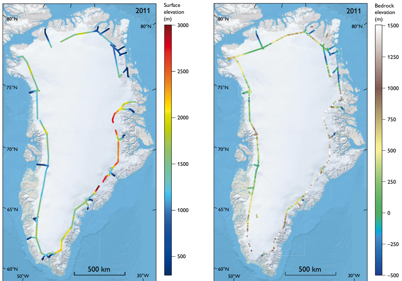
Fig. 2. A: Surface elevations along the PROMICE circum-Greenland flights in 2011. B: Bedrock elevations along the PROMICE circum-Greenland flights in 2011.
