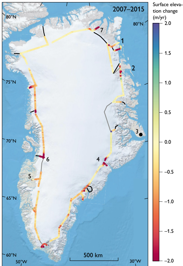
Fig. 3. Mean annual surface-elevation changes between 2007 and 2015 along the PROMICE circum-Greenland flight-paths. The part of the flight track for which only 2007 data are available is indicated in black, while 2015-only is indicated in grey. 1: Nioghalvfjærdsfjorden. 2: Storstrømmen. 3: Constable Pynt. 4: Kangerlussuaq Gletscher. 5: Kangerlussuaq. 6: Jakobshavn Isbræ. 7: Hagen Bræ.
