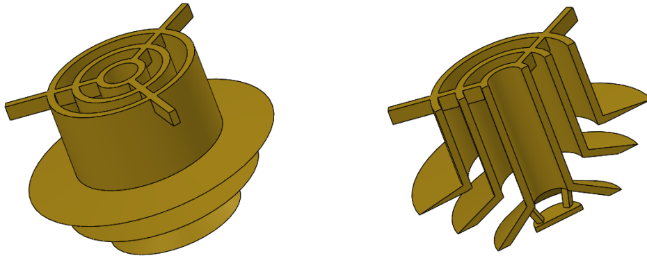
Fig. 2 Flow distributor/guide vanes, where it is possible to see the tripartite guide vane construction. It is mounted in the sudden expansion.
