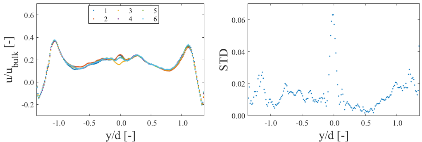
Fig. 11 Left: Velocity profiles from 6 independent run sampled at x/d = 2 , where the sampling frequency is at 7.26 Hz and the sample size are at 315 snapshots. The amplitude are 25% of the mean with a frequency at 1 Hz. Right: Standard deviation (STD) of the single points.
