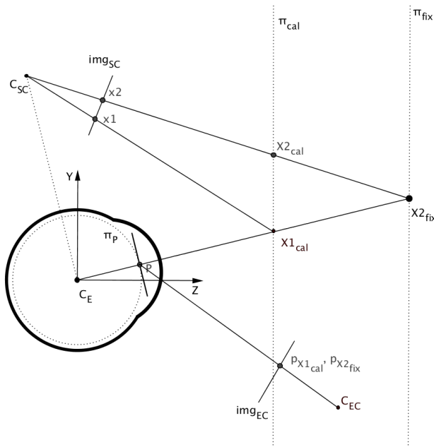
Figure 9. Sagittal view of a HMG T illustrating the epipolar geometry of the eye and the scene camera.
