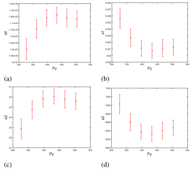
Figure 4. Relationship between the coefficients a_i of the regression function S_x against Y coordinate of the pupil center.
