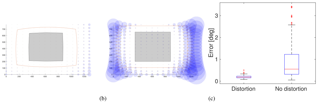
Figure 14. Gaze estimation error in the scene image showing the effect of radial distortion on polynomial function 1 ( 3 \times 3 calibration points) (a) with and (b) without lens distortion. The error in the working area for both conditions is shown in (c).
