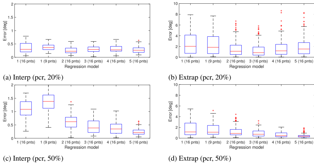
Figure 8. Gaze estimation error obtained from different regression models for interpolation and extrapolation regions of the scene image. Gaze estimation was based on the PCR feature and no measurement noise was applied to the eye image. Errors are measured in degrees.
