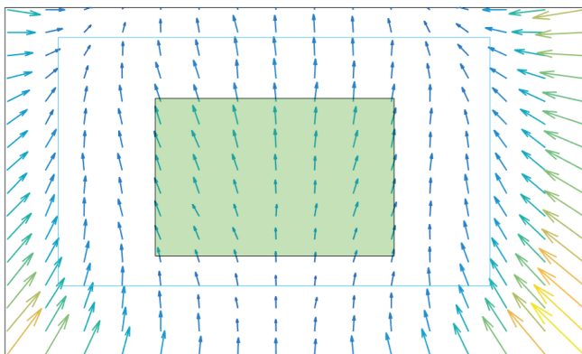
Figure 16. An example of error pattern in the image when having mapping error and parallax error combined
