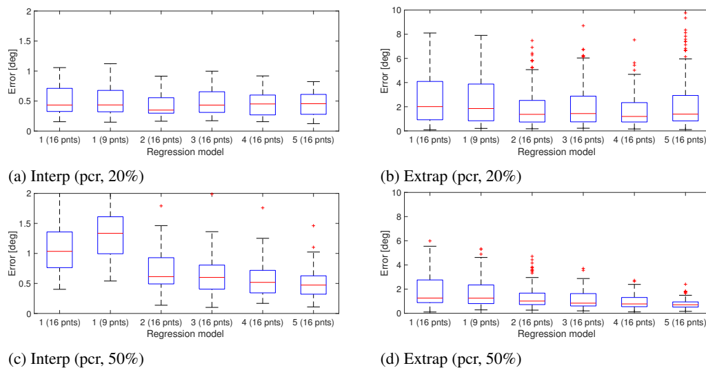
Figure 17. Gaze estimation error obtained from different polynomial models. Gaze estimation was based on the PCR feature. Resolution of the eye image is set to 1280 \times 960 and a noise level of 0.5 is applied. Errors are measured in degrees of visual angle.
