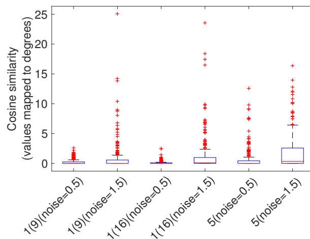
Figure 19. This figure shows how much different levels of measurement noise (in model 1 and 5) affects the direction of error vectors when having parallax error. The vertical axis represents the angular deviation.
