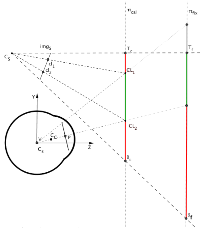
Figure 6. Sagittal view of a HMG
