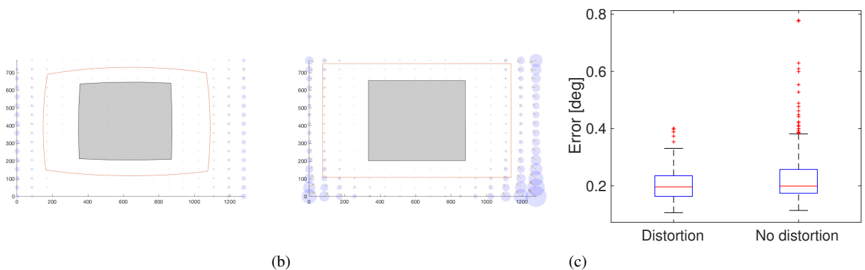
Figure 15. Gaze estimation error in the scene image showing the effect of radial distortion on polynomial function 5 ( 4 \times 4 calibration points) (a) with and (b) without lens distortion. The error in the working area for both conditions is shown in (c).
