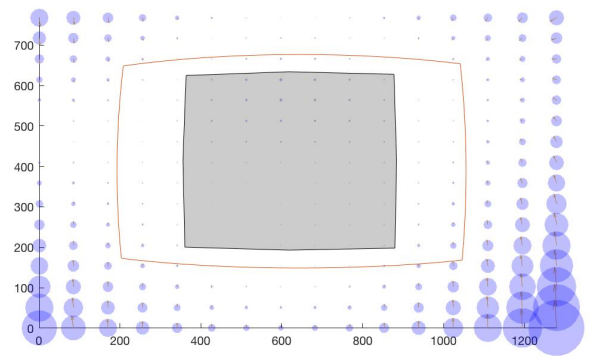
Figure 12. A sample image with radial distortion showing the calibration region (gray) and the working area (red curve).
