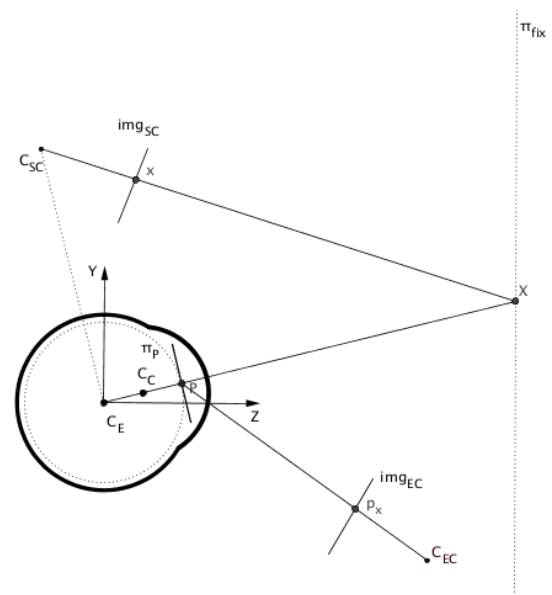
Figure 1. Sagittal view of a HMGT
