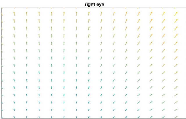
Figure 10. parallax error in the scene image for fixation distance at 3 m when d_{cal} = 1 m on the setup described in Table 2. This figure assumes an ideal mapping function with zero interpolation and extrapolation error in the entire image for the calibration distance d_{cal} .
