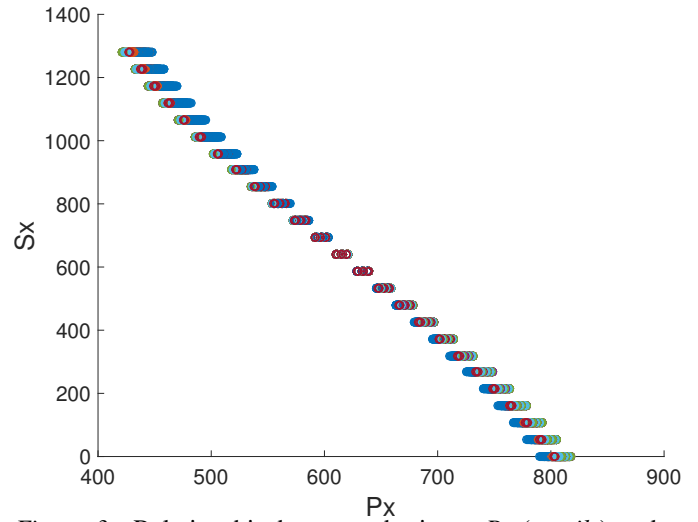
Figure 3. Relationship between the input P_x ( pupil_x ) and output ( S_x ). Different curves show the result for different parameters in the eye models.
