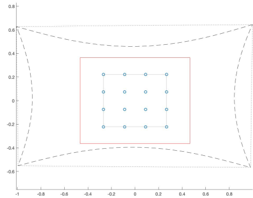
Figure 11. Calibration grid (small circles) and working area (red rectangle) marked in the calibration plane and borders of the scene image when it is back-projected onto the calibration plane with (dashed line) and without (dotted line) lens distortion. This figure was drawn according to the settings described in Table 5.
