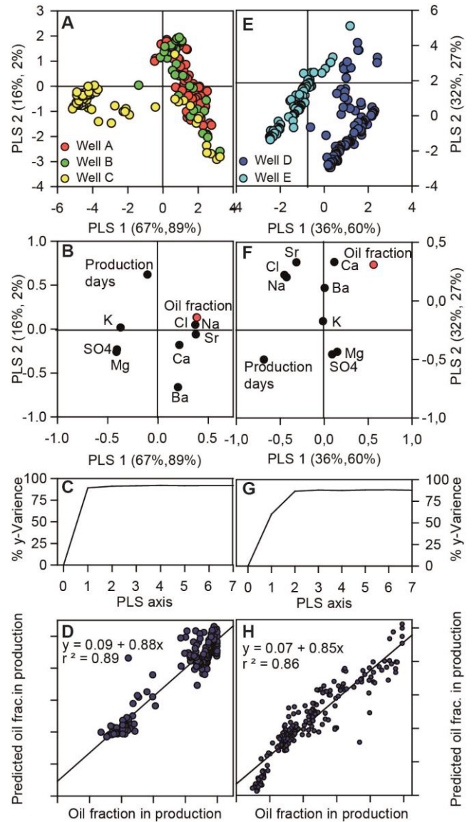
Fig. 6. PLS-regression model for well A, B and C (A-D) and well D and E (E-H) [water chemistry and production day, oil fraction in production] variable set; full training set. A and E: PLS X-space score plot (t1-t2). B and F: Corresponding loading-weights plot (w1-w2). C and G: Modelled y-variance. D and H: Prediction versus reference plot. Outliers were deleted from the original data set.
