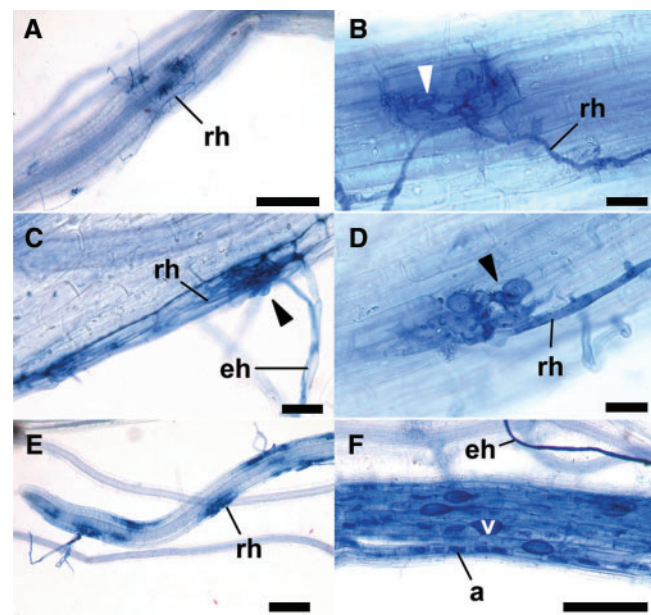
Fig. 2 AM symbiosis phenotypes of Ospollux and Osccamk mutants. Light micrographs of trypan blue-stained roots 6 wpi with G. intraradices are shown. AM structures are indicated by a, arbuscule; eh, external hypha; ih, internal hypha; rh, running hypha; and v, vesicle. Arrowheads indicate aberrant appressoria. Scale bars: A, E and F, 0.2 mm; B, C and D, 0.02 mm. (A and B) Osccamk mutant, NE1115. (C and D) Ospollux mutant allele, NC6423. (E) Ospollux mutant allele, ND5050. (F) Wild-type Nipponbare.
