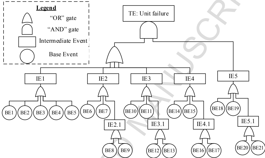
7 8 Fig. 7 Structure of FTA of ATUs in the case study 9
