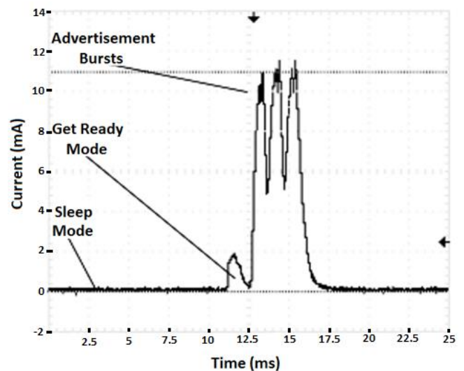
FIGURE 3. The measured SoC current, 2mA peak prior to BLE TX advertisement, three advertisement bursts at 11mA peak and 148uA static current in sleep mode (2 mA scale per vertical square and 2.5 ms scale per horizontal square).
