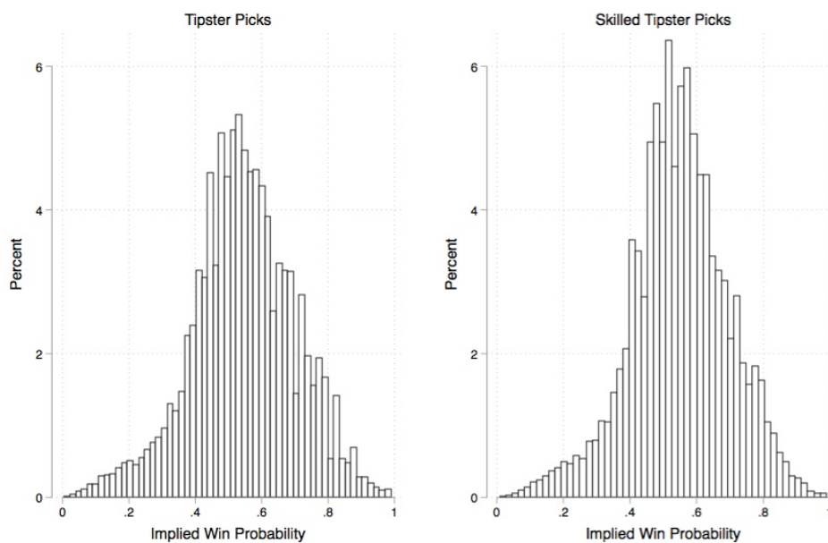
Figure 6: Histogram: Skilled Tipster Picks. Histograms of the implied win probability of bets picked out by tipsters (left), and bets picked out by skilled tipsters (right).
