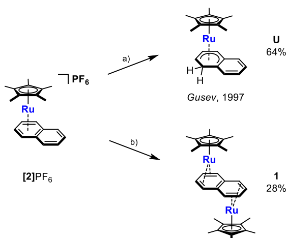
Scheme 1 Synthesis of complexes 1 and U ; 13 conditions and reagents: a) Na/Hg (excess), THF; b) KC_8 (1.1 equiv.) / -C_{10}H_8 , DME, 16 h, -30^\circ C to r.t.
