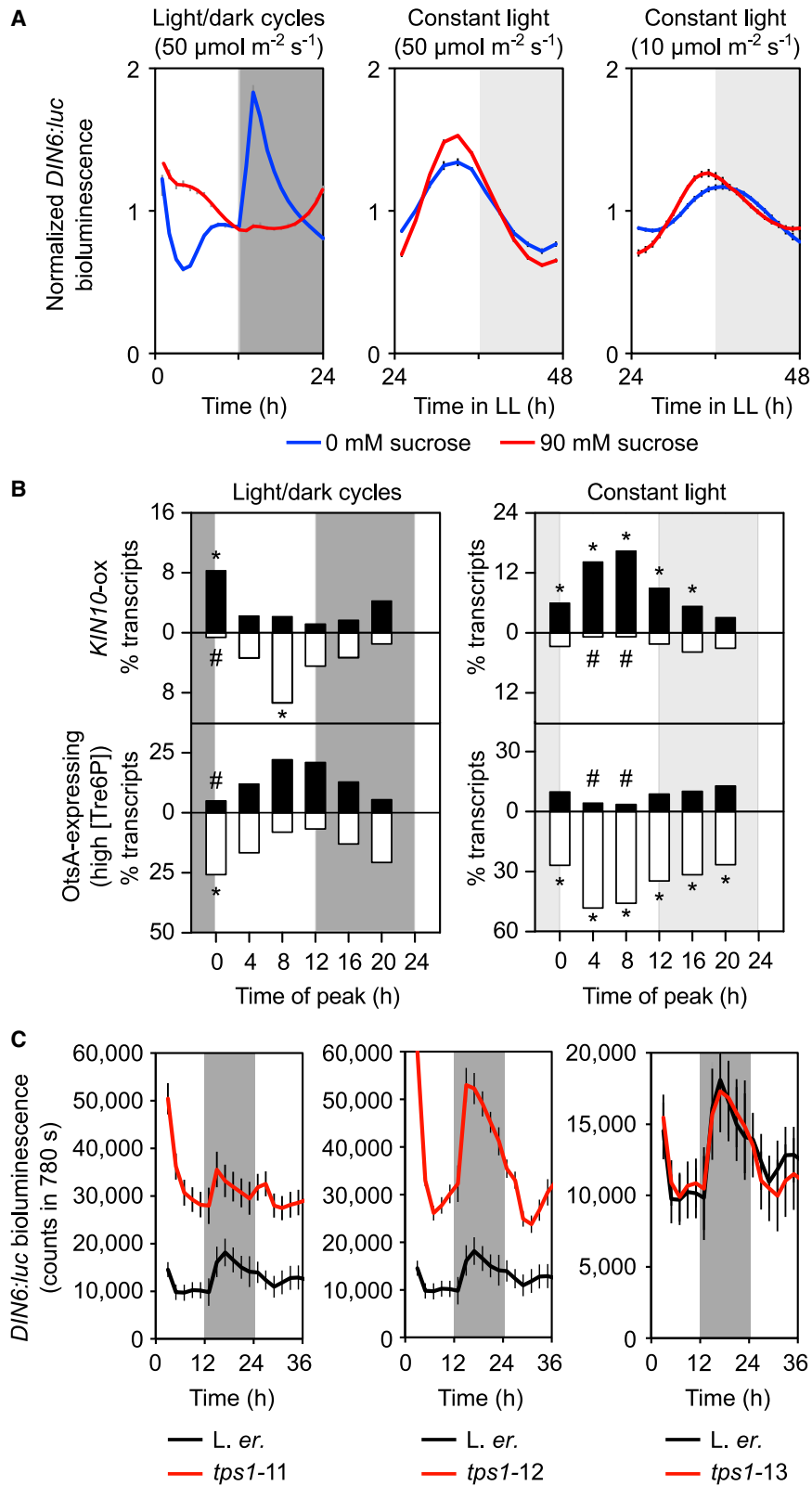
Figure 3. Diel Cellular Energy Signaling Dynamics
