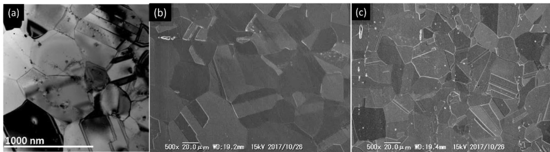
Fig. 5. Grain morphology of a) MA304LZ, b) SUS304L and c) SUS316L.
