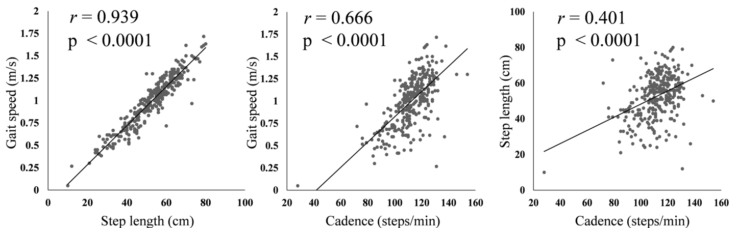
Fig 2. Correlations between three basic gait parameters. Correlation plot demonstrated the very strong, strong and moderate correlations between three basic gait parameters. r values = Pearson correlation coefficient.
