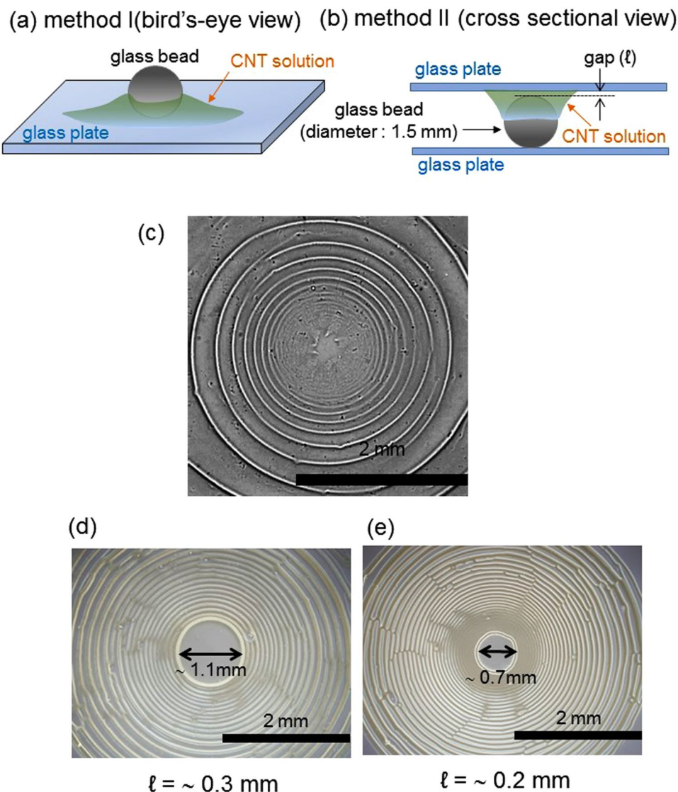
Figure 1. Schematics of two types of experimental setup (a,b) and drying patterns from the setups; (c) Pattern from Fig. 1a setup. (d,e) Patterns from Fig. 1b setup. The gap between the top of the glass bead and the upper glass plate, shown in Fig. 1b, is of different sizes in (d) and (e). The concentrations of PFO and SWCNT are 1.0 g/L and 0.33 g/L, respectively. A glass plate is used as the solid surface.
