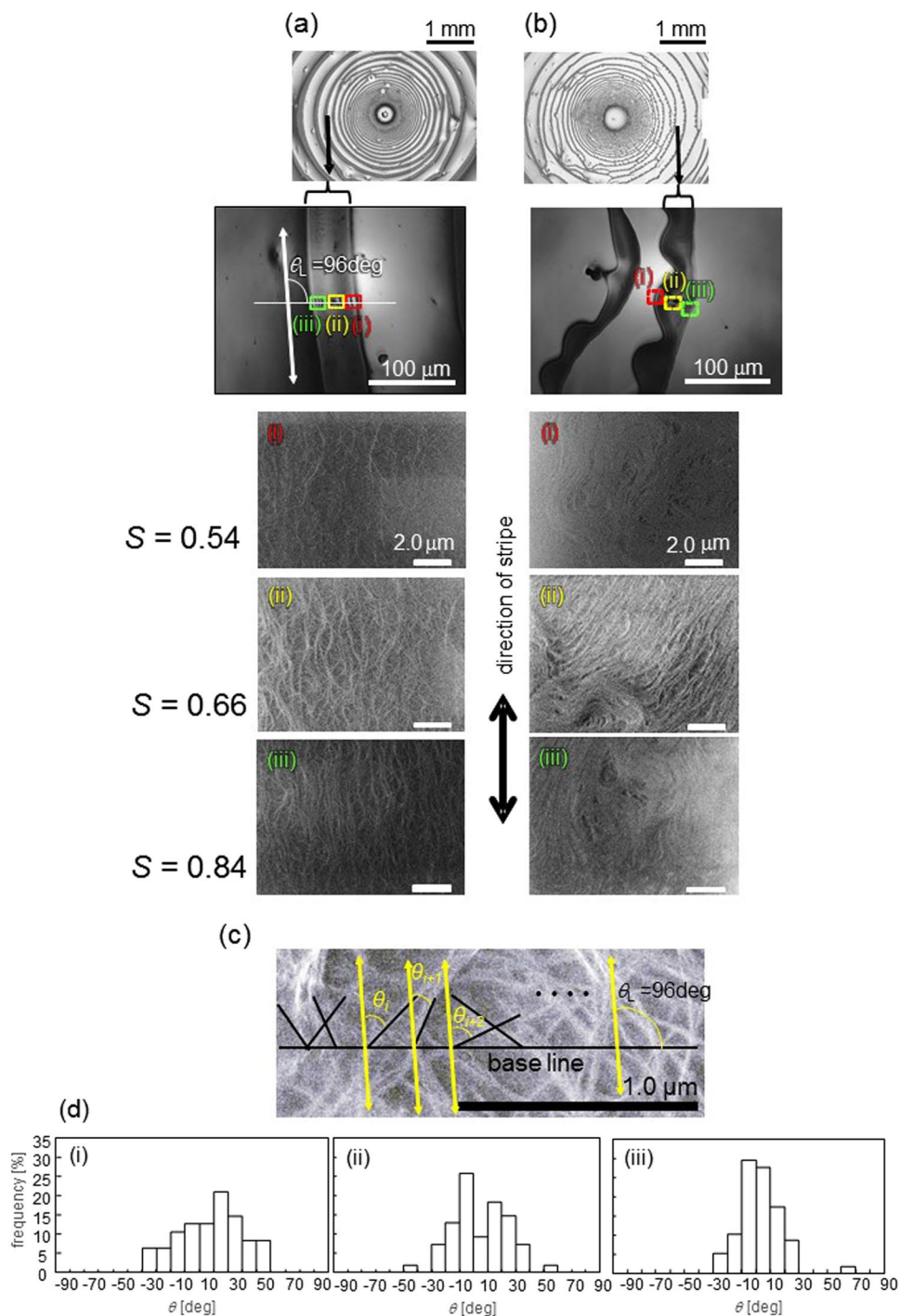
Figure 7. Scanning electron microscopy images of (a) smooth and (b) wavy patterns with quantification of ordering in SWCNT alignment (c,d). (a,b) The top two panels of each column are obtained by laser microscopy. The direction of the stripe is equal in the SEM and laser microscopy images. (c) Definition of \theta_i in eq. 1. The base and yellow oblique lines, respectively, are the same as those shown in (a). (d) Distribution of the angle calculated as \theta_i . The concentrations of PFO and SWCNT are 1.0 g/L and 0.33 g/L, respectively. A silicon wafer is used as the solid surface.
