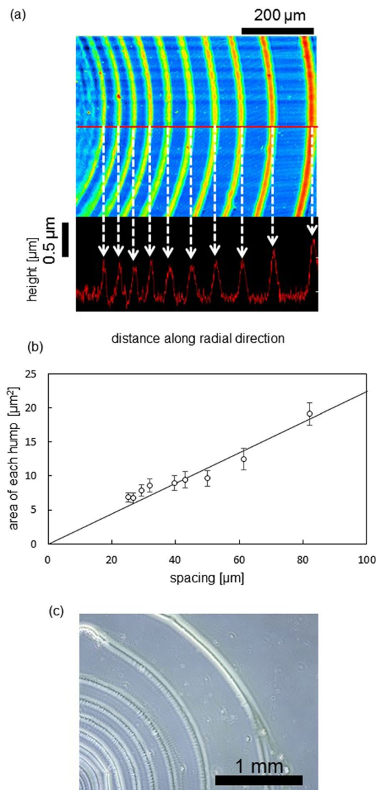
Figure 2. Laser microscopy image with height analysis of the drying pattern under atmosphere (a) and the spacing of stripes and the cross-sectional area of each hump (b) are shown. (c) An optical microscopy image of the drying pattern under vacuum. The concentrations of PFO and SWCNT are 1.0 g/L and 0.33 g/L, respectively. A glass plate is used as the solid surface.
