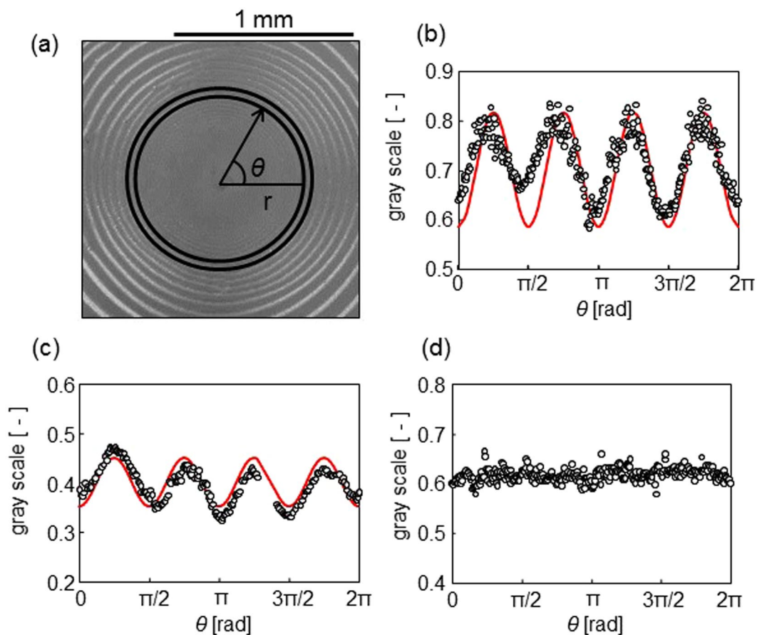
Figure 6. Polarized optical microscopy image of a drying pattern containing SWCNTs and PFO. (a) The micrograph on a glass surface. (b) and (c) show the gray scale as a function of the azimuth angle for the glass surface and silicon wafer, respectively. (d) Gray scale of optical microscopy image of PFO alone. The concentrations of PFO and SWCNT are 1.0 g/L and 0.33 g/L, respectively. For experiment of (d), SWCNT was not contained. A glass plate is used as the solid surface.
