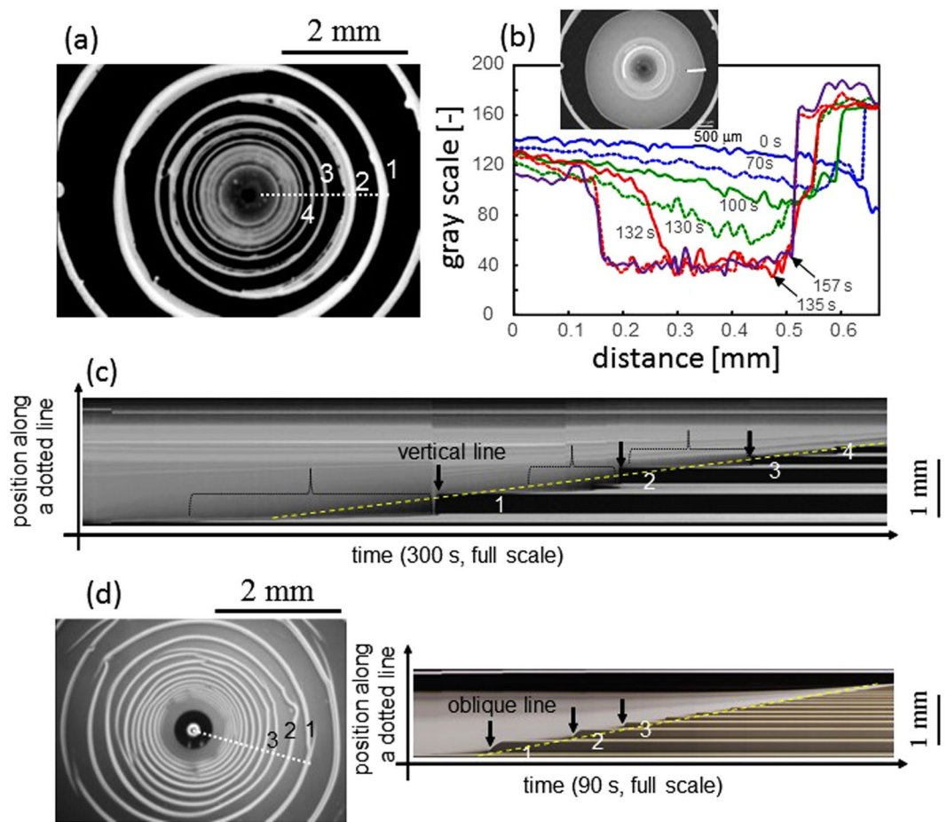
Figure 5. Dynamics of pattern formation. (a) Final fluorescence image of concentric-ring pattern. Glass coated by silicon is used as the solid surface. (b) Time-course of fluorescence intensity (gray scale of the photograph) along the line shown in the inset. A glass plate is used as the solid surface. (c) and (d) show, respectively, a space-time plot of pattern formation along the line shown in (a) and in the left image in (d). For both experiments, the concentrations of PFO and SWCNT are 1.0 g/L and 0.33 g/L, respectively.
