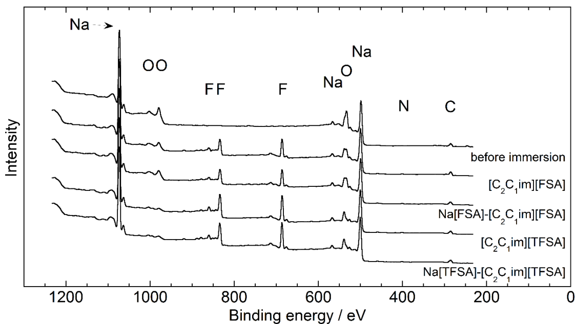
Figure 7 X-ray photoelectron spectra of Na metal before and after immersion in [\text{C}_2\text{C}_1\text{im}][\text{FSA}] , \text{Na}[\text{FSA}]-[\text{C}_2\text{C}_1\text{im}][\text{FSA}] (10:90), [\text{C}_2\text{C}_1\text{im}][\text{TFSA}] , and \text{Na}[\text{TFSA}]-[\text{C}_2\text{C}_1\text{im}][\text{TFSA}] (10:90) for one week. Etching time: 5 s.
