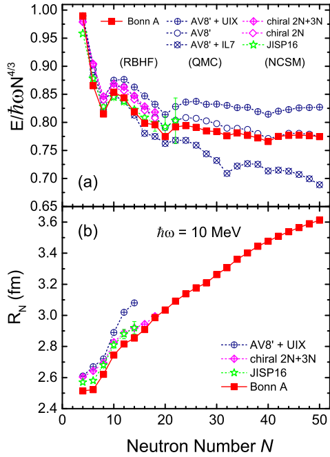
Fig. 1. (Color online) (a) Total energy divided by h\bar{\omega}N^{4/3} and (b) radii of N -neutron drops in a HO trap calculated by the RBHF theory using the interaction Bonn A [73], in comparison with other nonrelativistic ab initio calculations. See text for details.
