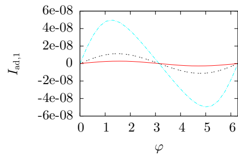
Fig. 3. (Color online) Adiabatic current I_{ad,1} in units of Ampère as a function of the difference between the phase of two gate fields for a driving frequency \omega = 4.13 \times 10^{12} Hz and different amplitudes V_{1,1} = 0.05 a.u. (solid red line), V_{1,1} = 0.1 a.u. (dashed black line), V_{1,1} = 0.2 a.u. (turquoise dash-dotted line); additional parameters: V_{0,1} = V_{0,2} = 0.54 a.u., L = 7.35 nm, m = 0.067 m_0 , \mu = 0.054 eV, T = 300 K.
