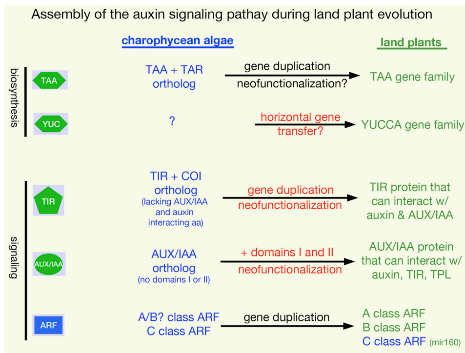
Figure S3. Summary of the Proposed Origins of Components of Auxin Biosynthesis and Signaling Components, Related to Figure 5
