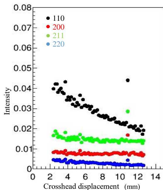
Figure 8. Change in diffraction intensity in the transverse direction
