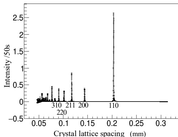
Figure 6. Diffraction pattern in the axial direction taken before deformation
