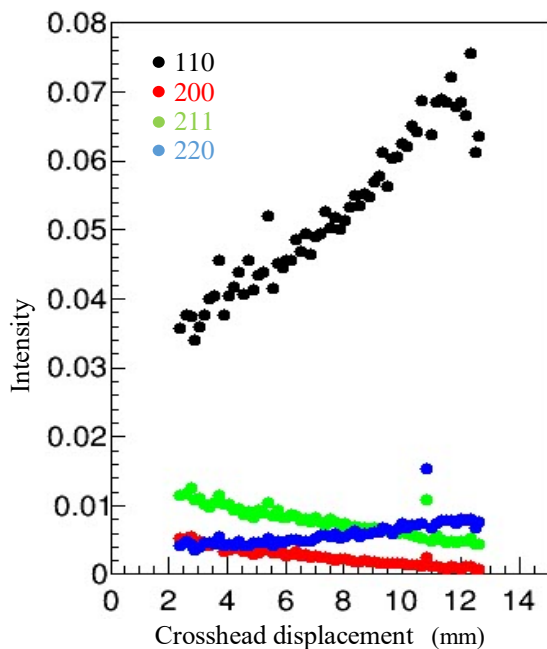
Figure 7. Change in diffraction intensity in the axial direction
