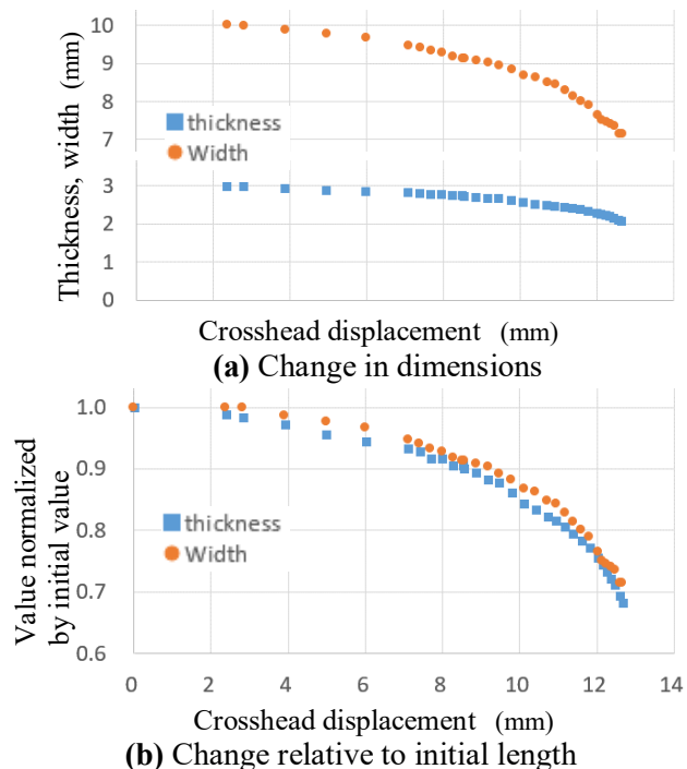
Figure 4. Changes in the thickness and width at the most reduced section of the specimen
