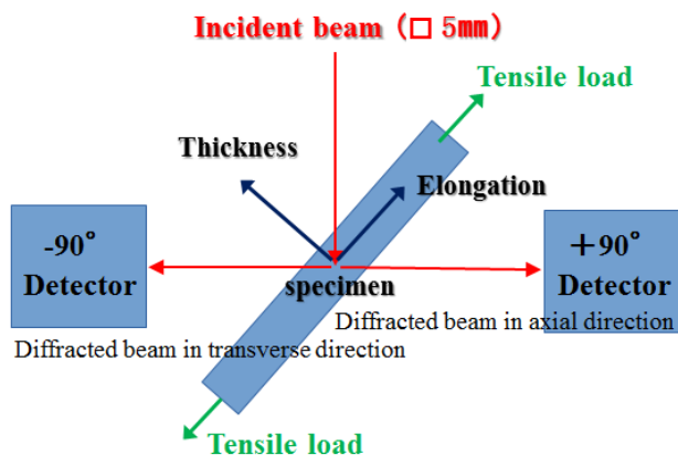
Figure 2. Schematic view of neutron diffraction measurement
