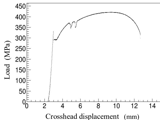
Figure 3. Load-crosshead displacement diagram
