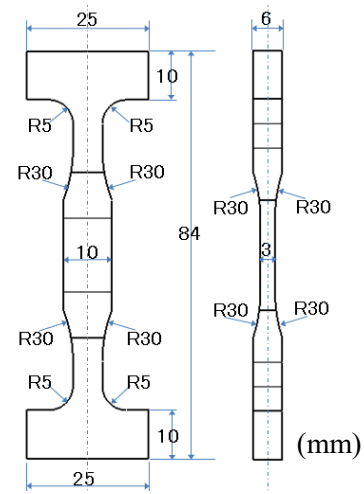
(a) Dimensions of a tensile specimen
