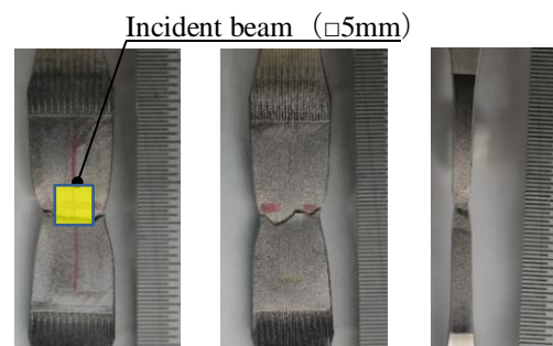
Figure 5. Photographs of specimen after fracture
