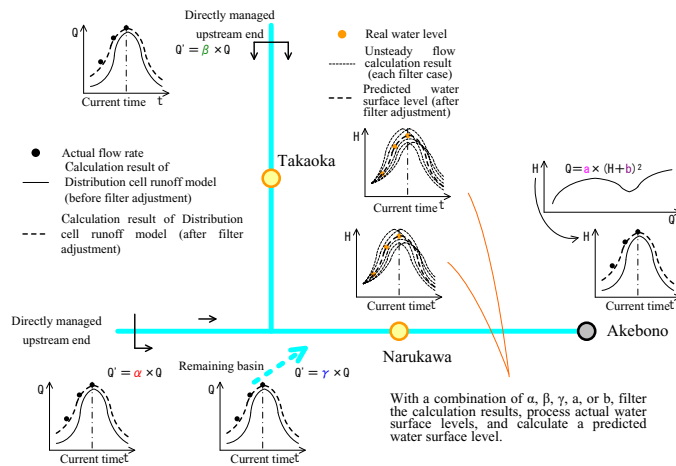
Fig.3 Outline of water surface level prediction model (Downstream end condition: HQ equation)
