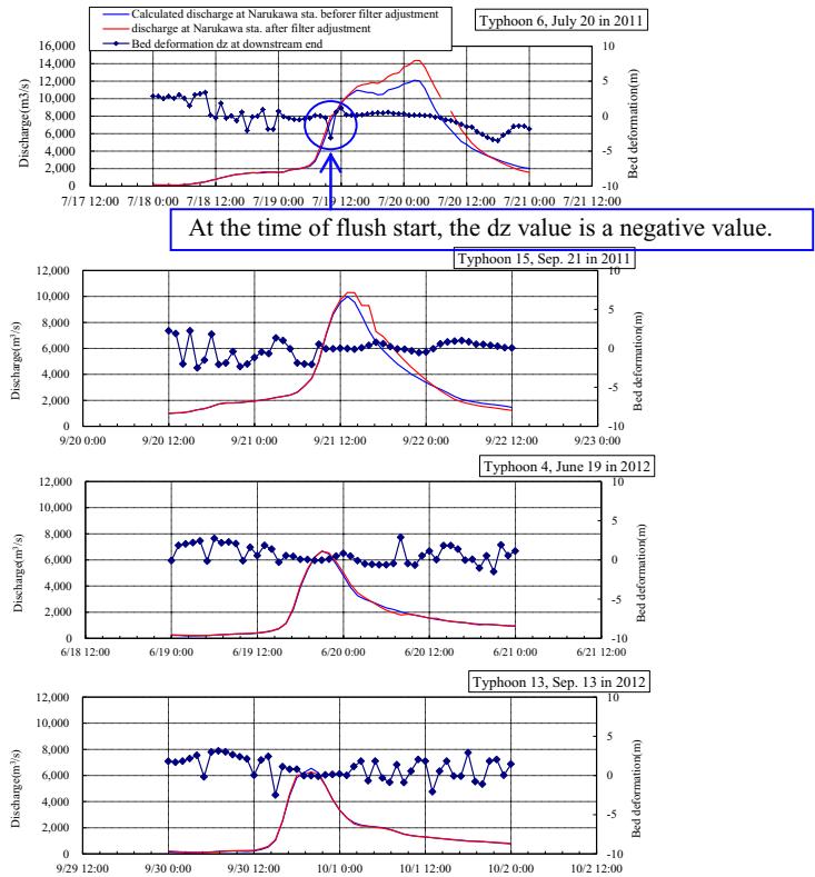
Fig.5 Time series change of state quantity
