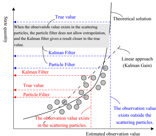
Fig.4 Difference between Kalman Gain and weight sampling
