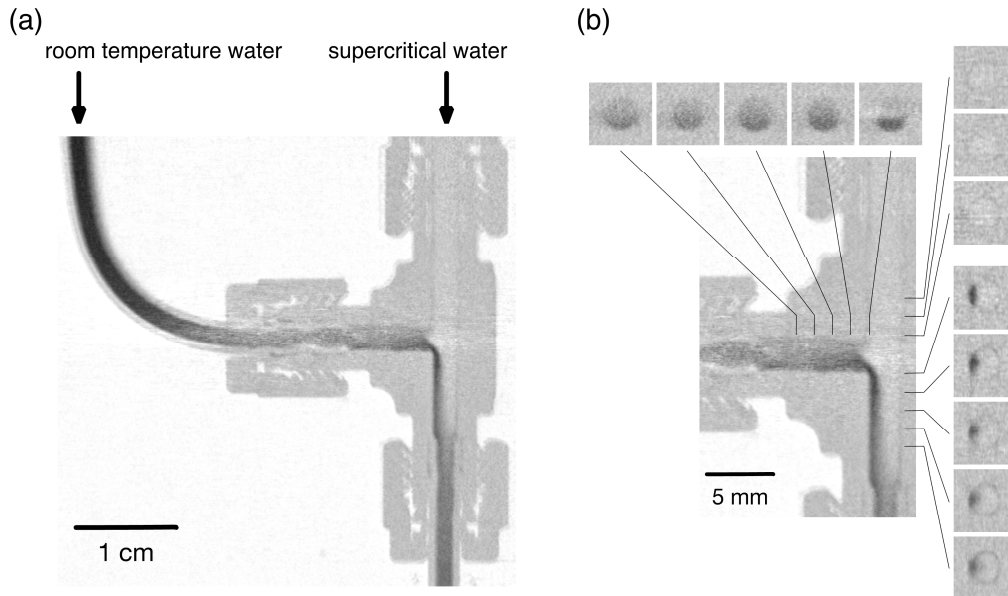
Fig. 3. (a) Reconstructed vertical cross sectional image of neutron attenuation at the center of mixing piece when supercritical water was supplied from top; (b) Horizontal cross sectional images around the mixing piece.
