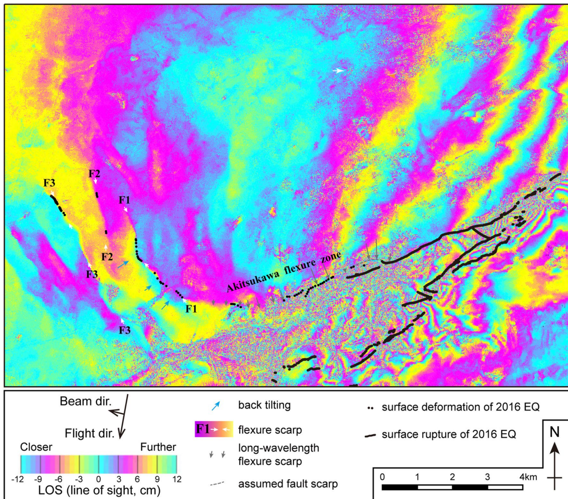
Fig. 6 Distribution of active faults and surface deformation associated with 2016 Kumamoto earthquake dropped over the InSAR deformation map, descending interferograms computed from ALOS-2/PALSAR-2 images of March 7, 2016, and April 18, 2016 (Geospatial Information Authority of Japan 2016a). The trace of surface ruptures associated with 2016 Kumamoto earthquake is after Kumahara et al. (2016)
