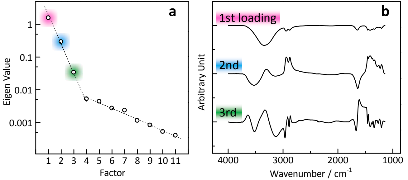
3 Fig. 2 Calculated results of the PCA analysis: (a) Eigenvalues, \lambda , plotted against the factor rank, i in a 4 semi-log graph. (b) First three loading vectors ( \mathbf{p}_i ; i = 1\sim 3 ).
