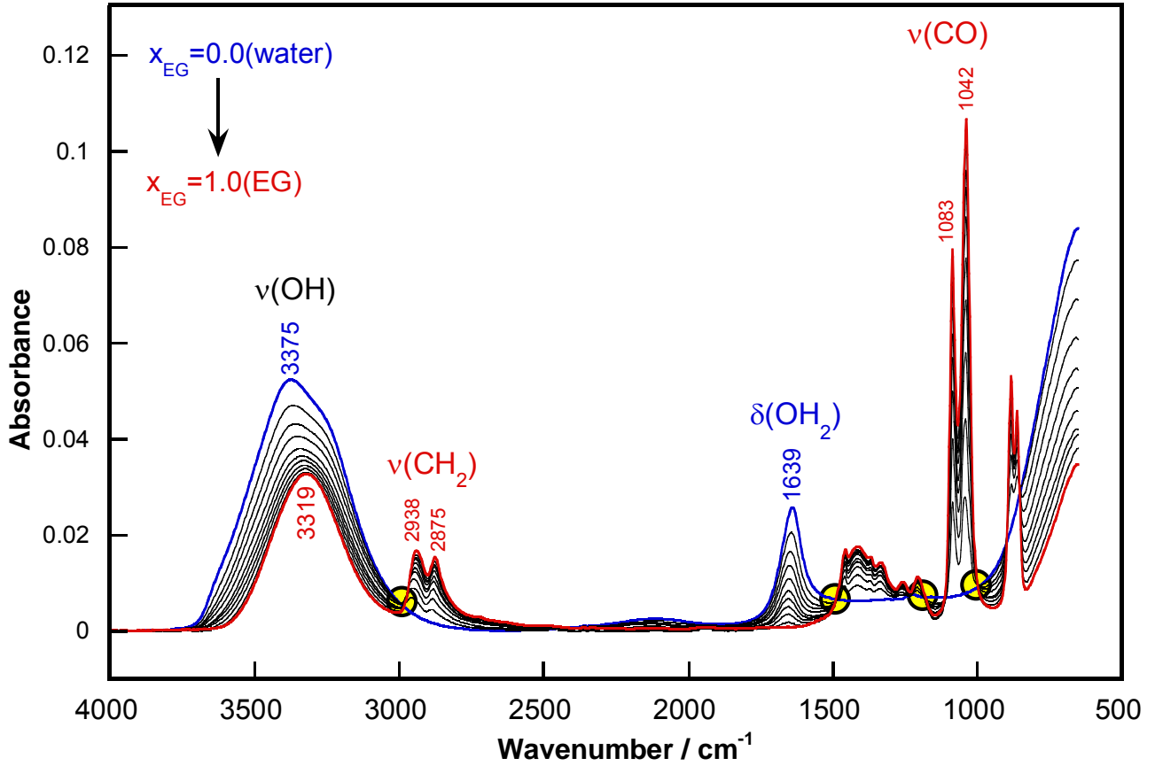
2 Fig. 1 Concentration dependent IR ATR spectra of the EG aqueous solution from x_{EG}=0.0 (pure water) 3 to 1.0 (pure EG). The yellow circles exhibit the isosbestic-like cross points.
