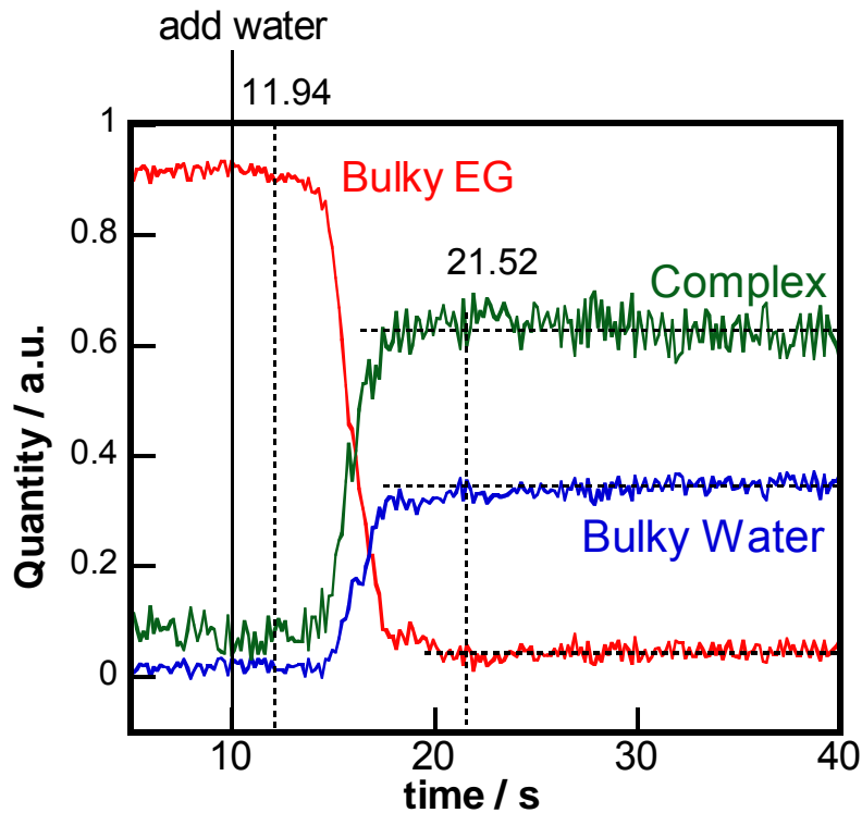
2 Fig. 7 The time-dependent quantities of the three constituents calculated by the CLS regression.
