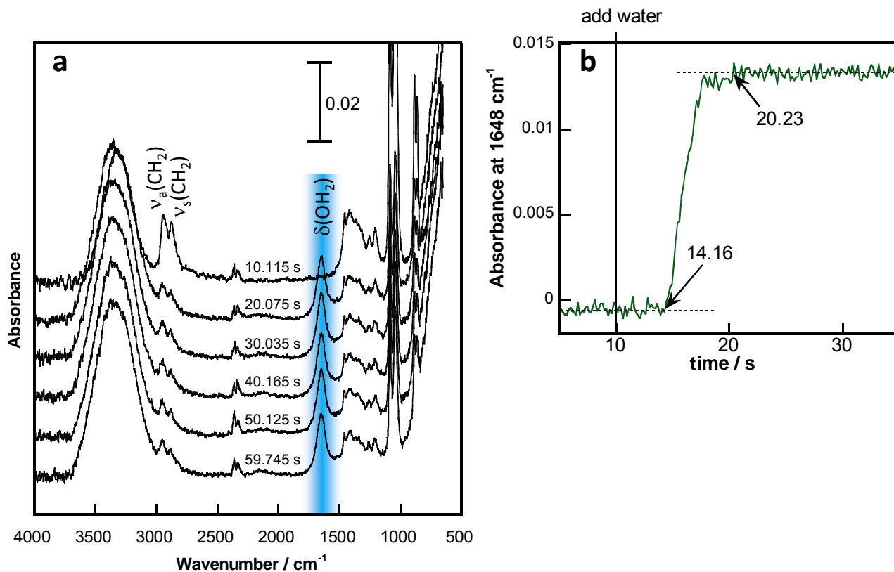
2 Fig. 5 (a) Selected time-resolved IR ATR spectra from 10.115 to 59.745 sec. (b) The time-dependent 3 absorbance at the \delta(\text{OH}_2) band of water at 1648 \text{ cm}^{-1} .
