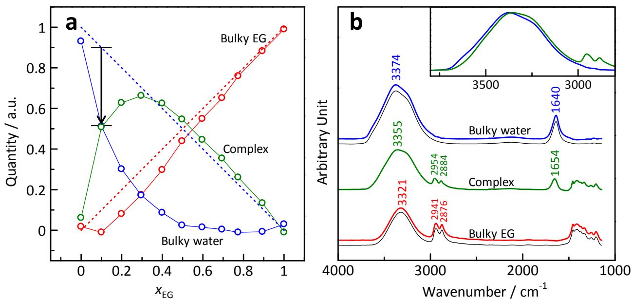
9 10 Fig. 3 (a) The quantity variations of the three constituents yielded by the ALS calculation: bulky water 11 (blue), bulky EG (red), and the complex (green), as a function of x_{EG} . Theoretical quantities of water 12 and EG in an ideal mixing are presented by the blue and red dotted lines, respectively. (b) The 13 corresponding spectra of the three constituents are presented with the same color as used in (a). Spectra 14 presented by black line beneath the blue and red ones are the spectra of pure water and EG, respectively. 15 The \nu(\text{OH}) bands of bulky water and the complex are overlaid in the inset.
