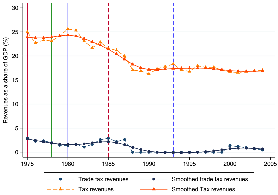
Figure 2: Definition of trade liberalization episodes and fiscal recovery: example of Chile
