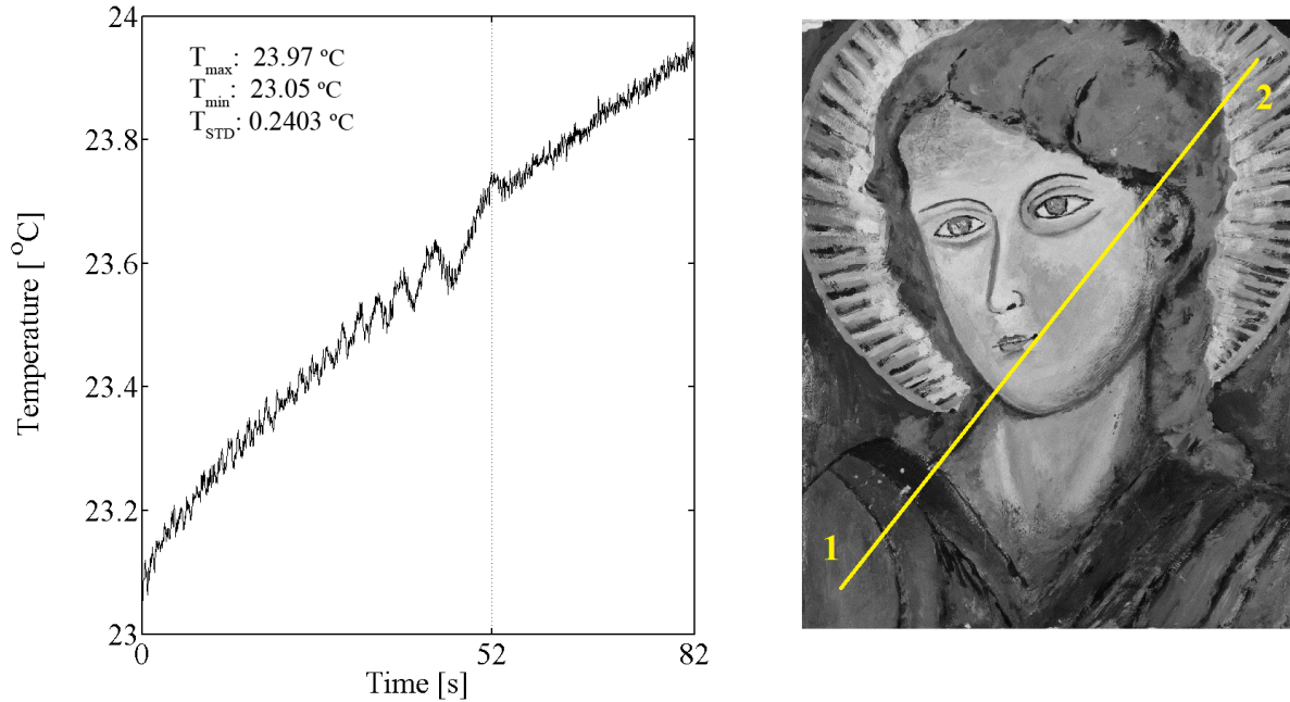
Fig. 7. Averaged temperature time handling of a line of pixels (1-2) crossing the panel painting surface while subject to the employed heating stimulus. Maximum ( T_{\max} ), minimum ( T_{\min} ) and standard deviation ( T_{\text{STD}} ) values are reported inside the plot.
