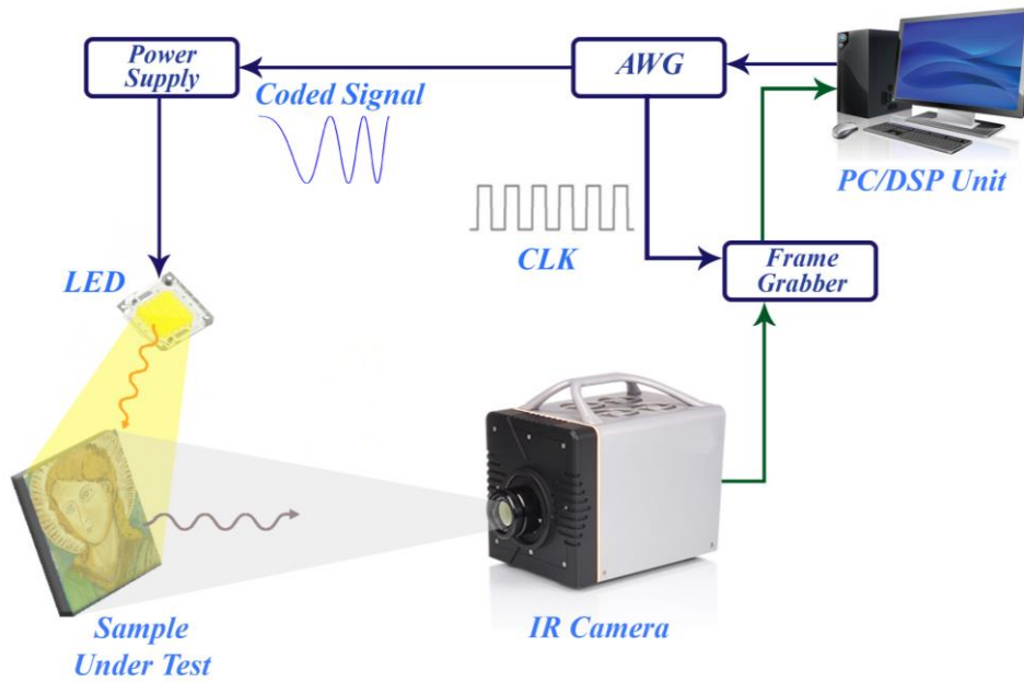
Fig. 6 The experimental setup. The Arbitrary Waveform Generator (AWG) and Frame Grabber were connected to a PC. The AWG board provided both the wanted linear chirp excitation and a reference clock signal (CLK) for triggering the IR camera acquisition. The coded signal was input into a TDK Lambda GEN 750W power supply that fed eight LED chips placed at about 30 cm from the sample under test.
