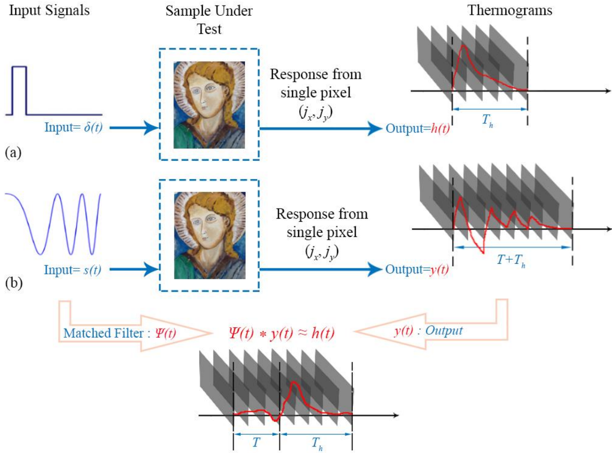
Fig. 3 Comparison between (a) Pulsed Thermography (PT) and (b) Pulse-Compression Thermography (PuCT). In PT the excitation is considered instantaneous and the sample impulse thermal response is measured for a time T_h , which is the impulse response time duration, i.e. the time necessary for the diffusion of the heat. In PuCT, the sample is excited with a coded excitation of duration T and thermograms are collected for an overall time duration of T+T_h . After the application of the PuC algorithm, an estimated impulse thermal response of duration T_h is retrieved.
