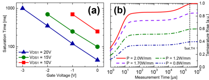
Fig. 5: (a) Saturation time of DEG2, t_{sat} , at V_{DS1} = 20V, 15V, and 10V and V_{GS1} = 0V to -3V ; showing the dependence of t_{sat} with both V_{DS1} and V_{GS1} . (b) transient heating at various power densities ( P ) using the RC thermal model [10], [19]. It is noted that t_{sat,TH} is temperature independent.
