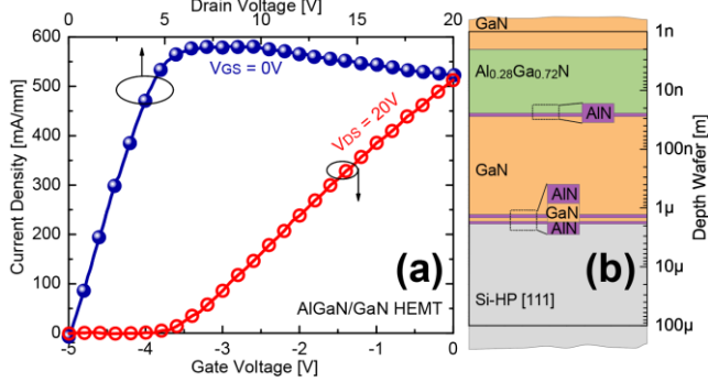
Fig. 1: (a) I_{\text{DS}}-V_{\text{DS}} and I_{\text{DS}}-V_{\text{GS}} characteristics at V_{\text{GS}}=0\text{V} and V_{\text{DS}}=20\text{V} , respectively, of the used AlGaIn/GaN HEMT. (b) Schematic cross-section of the epi-structures grown on Si-HP [111] substrate. The source-to-drain distance and device width are 5 \mu\text{m} and 100 \mu\text{m} , respectively.
