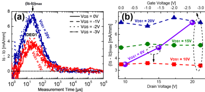
Fig. 4: (a) I_S and I_D difference ( I_S - I_D ) versus the measurement time at V_{DS1} = 20V and 10V for different gate voltages ( V_{GS1} = 0V to -3V ); indicating the bulk trapping process (DEG1). (b) The impact of drain voltage, V_{DS1} , and gate voltage, V_{GS1} on (I_S - I_D)_{max} given at t \approx 30\mu s ; unlike V_{DS1} , V_{GS1} shows a negligible impact on bulk trapping characteristics.
