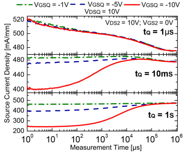
Fig. 6: Recovery of current, measured at V_{DS2} = 10V and V_{GS2} = 0V (Fig. 2b), after various pre-charging conditions are applied: V_{GSQ} = -1V, -5V, and -10V , at V_{DSQ} = 10V , for a period t_0 = 1\mu s, 10ms, and 1s . The recovery in the current transients at t_0 \geq 10ms shows the dominance of surface trapping on device degradation over self-heating.
