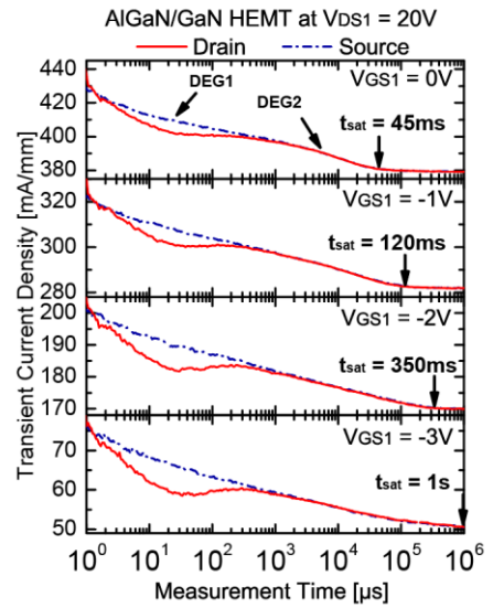
Fig. 3: Transient behavior of the drain, I_{\text{D}} , and source, I_{\text{S}} , currents, versus measurement time on log scale using the pulse waveforms given in Fig. 2a with V_{\text{DS1}}=20\text{V} , at V_{\text{GS1}}=0\text{V} to -3\text{V} . Two degradations of current are observed at different time constants, DEG1 and DEG2.
