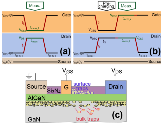
Fig. 2: Pulse waveforms used for I_{\text{S}} and I_{\text{D}} transient measurements for: (a) without traps pre-charging and (b) with traps pre-charging, where t_{\text{RESET}}=10\text{s} and t_{\text{E}}=200\text{ns} . (c) The schematic diagram of bulk and surface trapping mechanisms are illustrated for a semi-ON-state at V_{\text{DS}}>0\text{V} .
