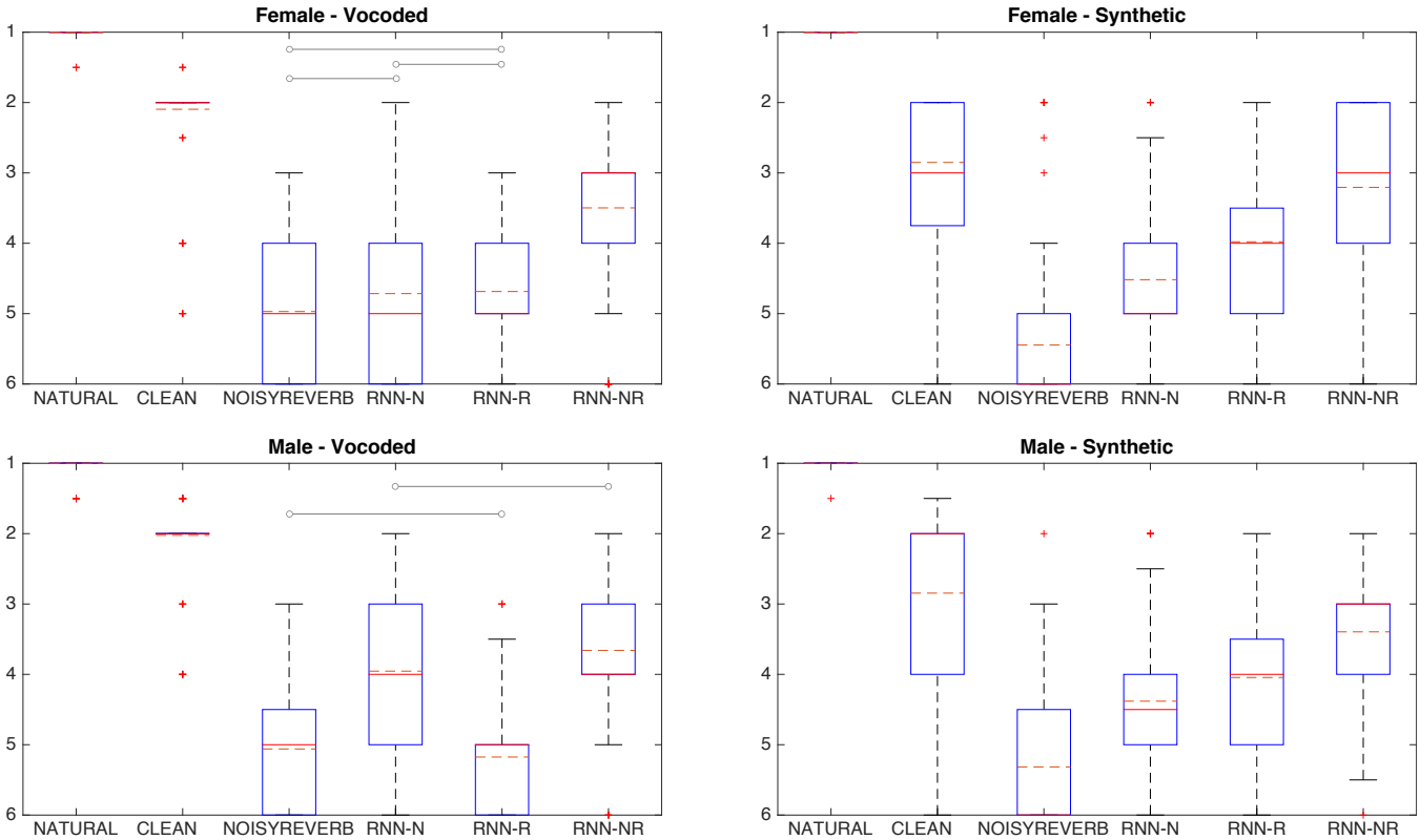
Fig. 5. Noisy and reverberant data evaluation: rank order values for vocoded (left) and synthetic (right) speech of female (top) and male (bottom).
