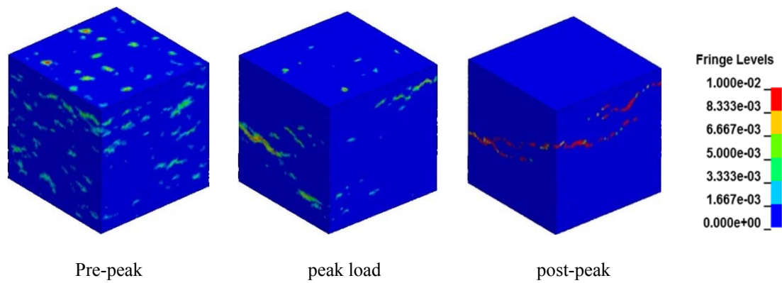
Fig. 14. Development of crack patterns
