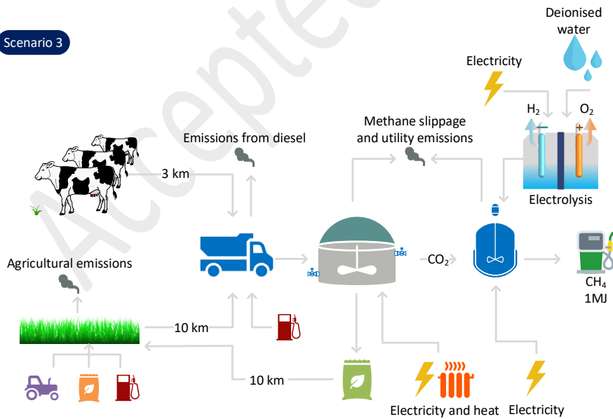
Figure 1: System boundaries of three scenarios
