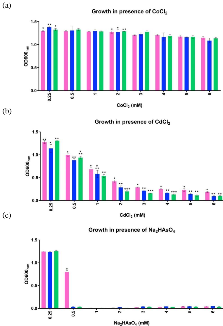
Figure 4: Growth of three strains of Lactobacillus paracasei in MRS supplemented with corresponding heavy metal salt (a) CoCl 2 , (b) CdCl 2 and (c) Na 2 AsO 4 , inoculated in concentration 1 % (w/v) and incubated over 48 h at 30°C. Bars represent OD 600nm . Bars for the same heavy metal salt concentration sharing the same asterisk symbol show no statistical difference in growth ( p>0.05 ), after mean comparison by performing One-way Analysis of Variance (ANOVA) followed by Least Significant Test (LSD). Error bars present standard deviation.
