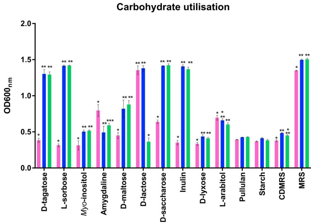
Figure 3: Growth of three strains of Lactobacillus paracasei in reconstituted MRS (CDMRS) supplemented with a single sugar in concentration 1 % (w/v) and incubated over 48 h at 30°C. Bars represent OD 600nm at the end of 48 h. Bars for the same sugar sharing the same asterix symbol show no statistical difference in growth ( p>0.05 ), after mean comparison by performing One-way Analysis of Variance (ANOVA) followed by Least Significant Test (LSD). Error bars present standard deviation.
