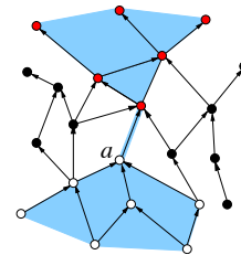
(b) Past and future causal cone the event a in customary causal-network representation.
