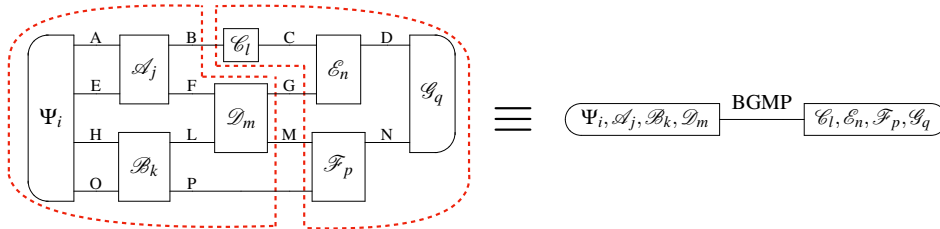
Figure 2: Every closed circuit is equivalent to composing a preparation with an observation.
