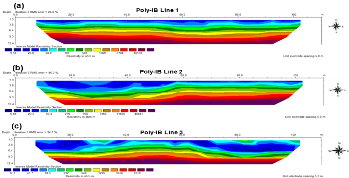
Fig. 5: 2D inverse resistivity model for Poly-IB profiles 1, 2 and 3.
