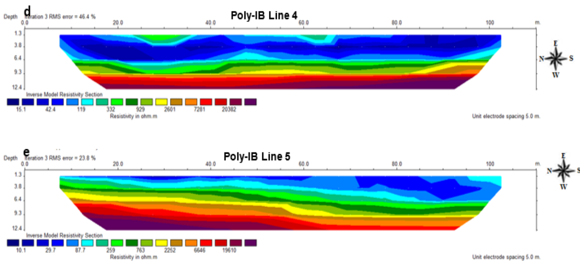
Fig. 6 2D inverse model resistivity sections for Poly-IB profiles 4 and 5.
