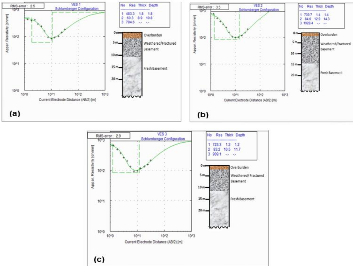
Fig. 3: VES curves and geoelectrical parameters obtained for (a) VES 1, (b) VES 2 and (c) VES 3.
