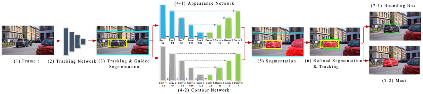
Figure 2: Tracking-assisted Weakly Supervised Segmentation Framework: (1) Input frame t . (2) A general tracking module, adopted from ECO [10]. (3) The tracker first helps to guide the segmentation. The yellow bounding box represents the predicted target position and size by tracker, while the cyan bounding box represents the area that is cropped for segmentation. (4) Segmentation module contains appearance network and contour network. (5) Initial segmentation results indicating with the red mask. (6) Tracking output and segmentation results help refine each other mutually. (7) Finally, two outputs are given, a bounding box for tracking, and a mask for segmentation. Best viewed in color.
