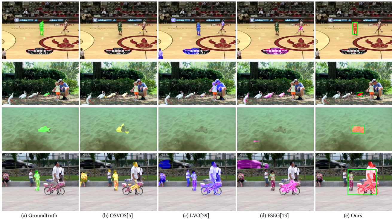
Figure 4: Illustration of Segmentation Results on the VOT2016 pixel-wise annotation: Green rectangle represents bounding box that tracker generate to help guide segmentation task. Our framework outperforms both semi-supervised and unsupervised methods. But the failure of tracker is prone to affect the performance of segmentation, for example in the last row, the tracker failed to follow the girl but follows another man, causing the segmentation to lose the target. Best viewed in color.
