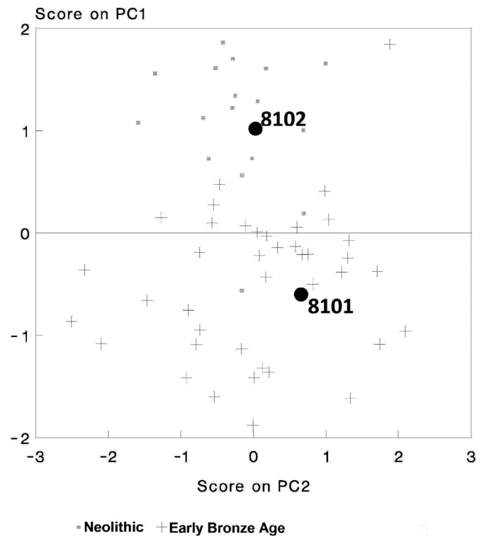
Fig. 10. Principle components analysis of cranial morphology of Neolithic and early Bronze Age crania using size corrected variables. Scatterplot of first and second principle components, with Middle Bronze Age crania of 8101 and 8102 superimposed.
