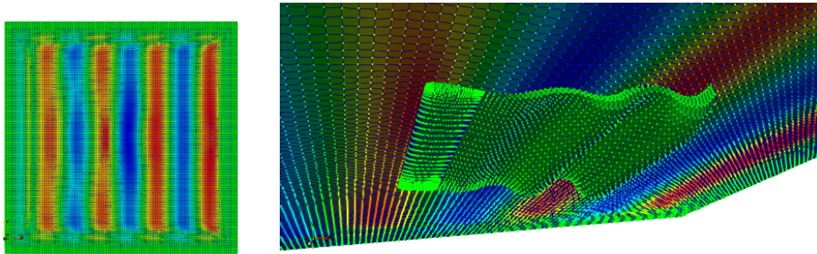
Figure 6: Wakedeformation. Dir 0
