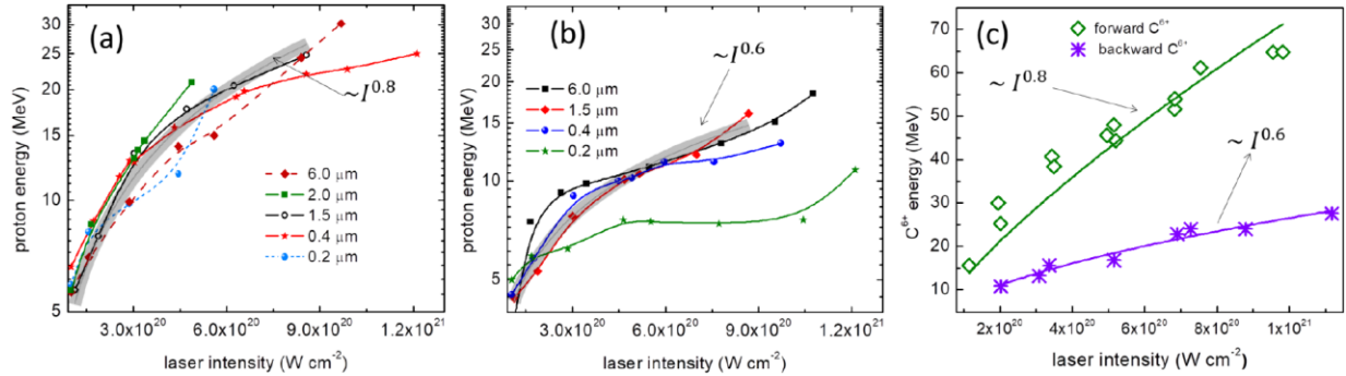
Fig. 4. Intensity scaling of proton and Carbon ions. Intensity dependent proton cut-off energy for different thickness of Al foil target is plotted for a) forward and b) backward direction. The thick grey line is the fitted curve on 1.5 \mu\text{m} data, representing intensity dependence of proton energies a) E_{\text{forward}} \propto I^{0.8} and b) E_{\text{backward}} \propto I^{0.6} for forward and backward accelerated proton, respectively. c) Intensity dependent \text{C}^{6+} cut-off energy is plotted for forward and backward direction. The solid lines are the fitted curve, representing intensity dependence of ion energies E_{\text{forward}} \propto I^{0.8} and E_{\text{backward}} \propto I^{0.6} for forward and backward \text{C}^{6+} , respectively.
