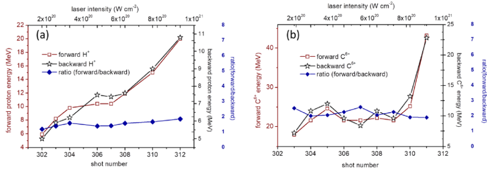
Fig. 2. Forward backward correlation for proton and Carbon ions. Maximum energy of accelerated ions from 0.2 \mu\text{m} thick \text{Al} target measured in arbitrary consecutive laser shots along the forward and backward direction for a) proton and b) \text{C}^{6+} ions where laser intensity is ramped up. The ratio of forward and backward maximum energy is shown by blue diamond.
