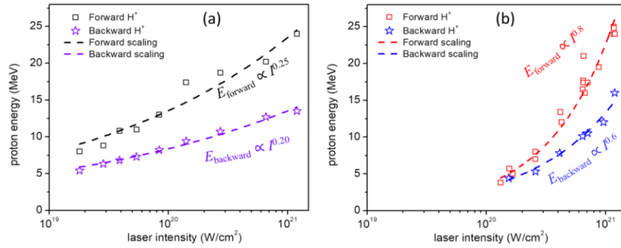
Fig.5. Proton intensity scaling with changing laser focal spot vs laser energy. Intensity dependent proton maximum energy scaling obtained under a) variation of the laser focal spot and b) by changing laser energy.
