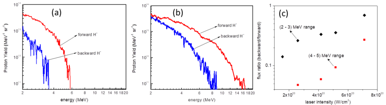
Fig. 3. Flux comparison of forward and backward protons. Kinetic energy spectrum of forward and backward accelerated protons for intensity of a) 1.5 \times 10^{20} \text{ W/cm}^2 b) 7.2 \times 10^{20} \text{ W/cm}^2 . c) Variation of backward and forward proton flux ratio in the energy range of (2.0 - 3.0) MeV and (4.0 - 5.0) MeV
