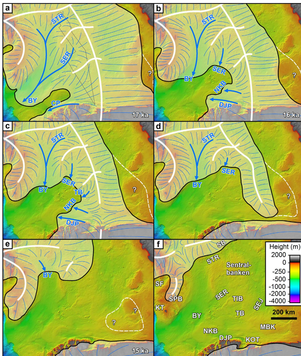
Fig. 11. (a–f) Time-slice reconstruction of the Barents Sea Ice Sheet between 17 and 14 ka. In panels with dates the ice sheet margin is the ‘most-credible’ reconstruction from Hughes et al. (2016). The ice margins and flow patterns have been generalised from studies discussed in the main text and from this study. White lines indicate possible locations of ice divides, whilst blue arrows and lines indicate ice streams and general flowlines, respectively. These are necessarily schematic due to the limited availability of data and are based on correlations across different sets of geomorphological data. Thus, this reconstruction provides a simplified pattern of retreat after ice streams reduced ice volume in the saddle area before the eventual separation of the Barents Sea Ice Sheet from the Fennoscandian Ice Sheet. The question marks refer to uncertainty in ice margin extent in the southeastern Barents Sea and a proposal for greater ice cover extent in the central and eastern Barents Sea. Abbreviations are the same as Fig. 1 except for coast-parallel ice stream (CP), Murmanskbanken (MBK), and Sentraldjupet (SEJ). See Fig. 2 for location. (For interpretation of the references to colour in this figure legend, the reader is referred to the web version of this article.)
