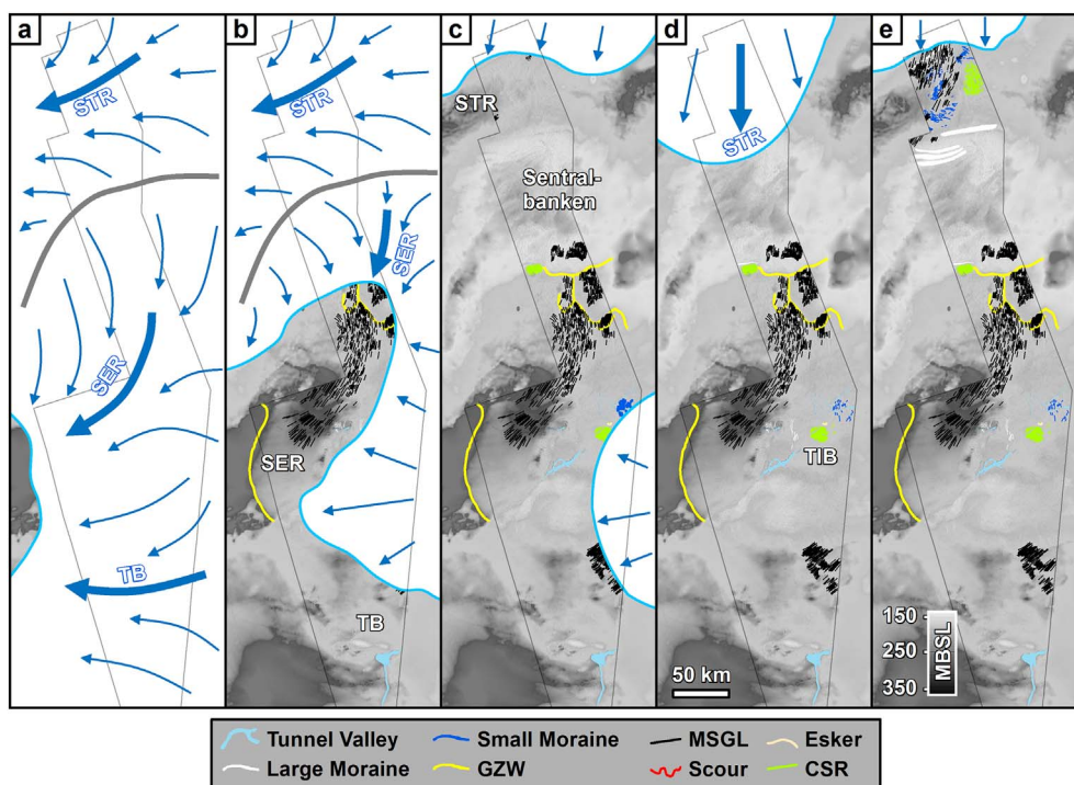
Fig. 10. Reconstruction of the demise of the central part of the BSIS across a number of tentative time-slices between 16 and 14 ka (a–e). Ice sheet margins and flowlines are based on the landform analysis in this paper, as well as published work on the adjacent areas (Winsborrow et al., 2010; Bjarnadóttir et al., 2014) but are necessarily schematic for areas due to the lack of dating control with which to constrain the chronology. The landform records that have been left behind after each event are also overlain onto the bathymetry. The white polygon marks the ice sheet extent and the thick blue arrows show areas where evidence for fast-flowing ice is observed. The thinner blue arrows show a generalised ice flow pattern based on the landform analysis, as well as an intuitive interpretation of the likely ice flow patterns in response to the topographical setting. The grey lines highlight possible ice divide locations that honour these flow patterns. Abbreviations are the same as for Figs. 1 and 9. The blue outlined abbreviations are the same but refer to the ice streams discussed in the text. See Fig. 2 for location. (For interpretation of the references to colour in this figure legend, the reader is referred to the web version of this article.)
