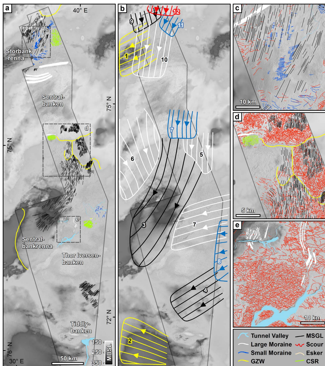
Fig. 9. a) detailed bathymetry overlay onto regional IBCAO v.3.0 bathymetry (Jakobsson et al., 2012b). The large-scale record of landforms is presented without iceberg scours for clarity due to the large number that are present; b) generalised flow-sets derived from the geomorphological record - descriptions and rationale of each flow-set are described in Table 1. The colours of the flow-sets are to allow differentiation of each flow-set and do not imply a link to other flow-sets with the same colour; c) enlarged image of the landform assemblage in the Storbankrenna; d) enlarged map showing retreating grounding-zone wedges in Sentralbankrenna; e) enlarged image of features on Thor Iversen-banken; cross-cutting of flow-sets represent the relative chronology of each set of landforms. Abbreviations are as follows: crevasse-squeeze ridges (CSR), grounding-zone wedge (GZW), and mega-scale glacial lineation (MSGL). (For interpretation of the references to colour in this figure legend, the reader is referred to the web version of this article.)
