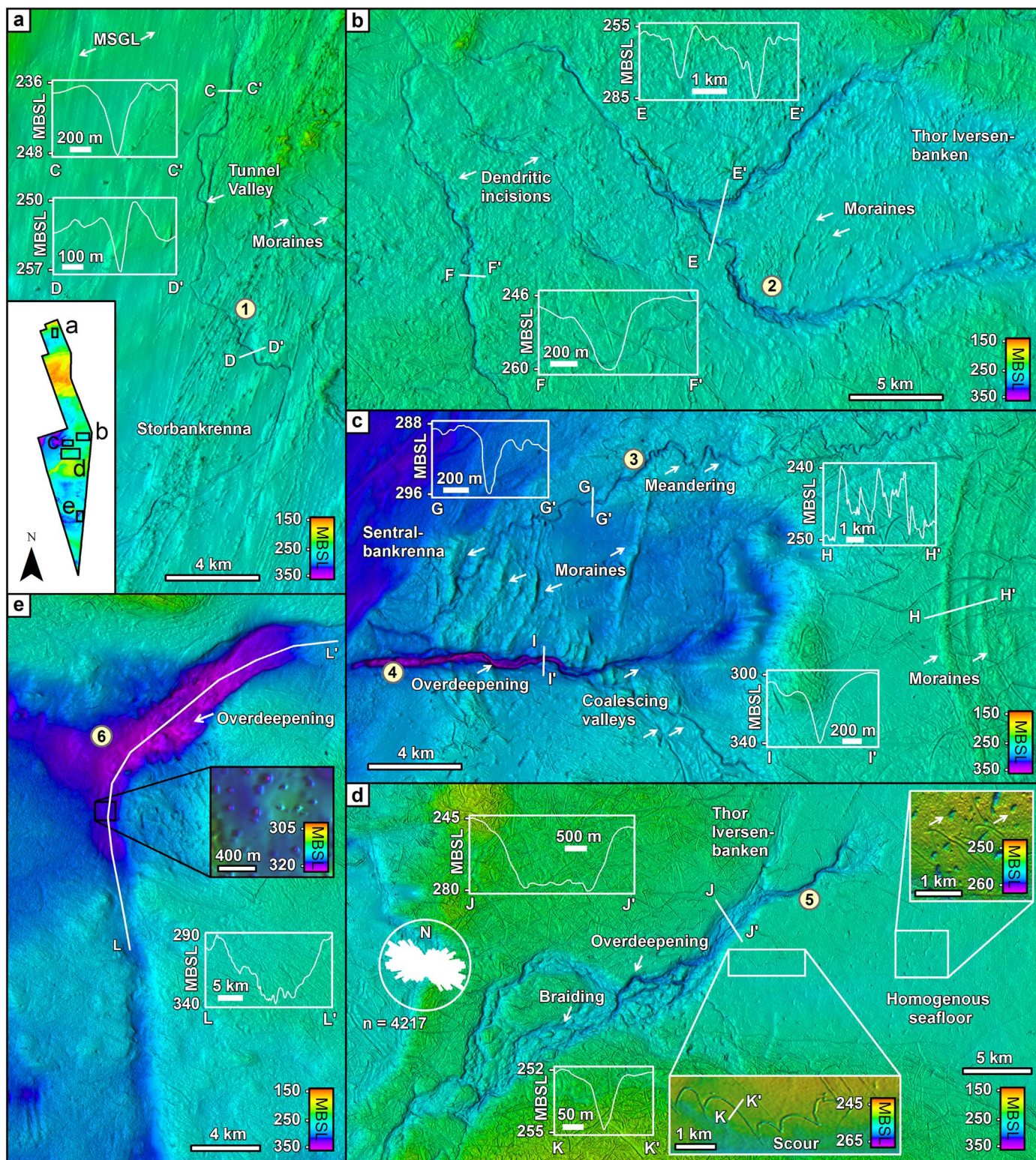
Fig. 5. Multiple examples of tunnel valleys and profiles across the survey area; a) tunnel valley 1 (TV-1) with associated MSGLs and retreat moraines in Storbankrenna; b) TV-2 and its tributary network on Thor Iversen-banken. Retreat moraines are also observed; c) the smaller valley in the north is TV-3 and the larger, overdeepened valley in the south is TV-4. Multiple retreat moraines are also observed on Thor Iversen-banken and are indicated by the white arrows; d) TV-5 on the southern part of Thor Iversen-banken. Inset panels show a curvilinear iceberg scour and observations of iceberg grounding pits; e) TV-6 is located between Thor Iversen-banken and Tiddlybanken. The inset panel shows observations of pockmarks associated with fluid expulsion.
