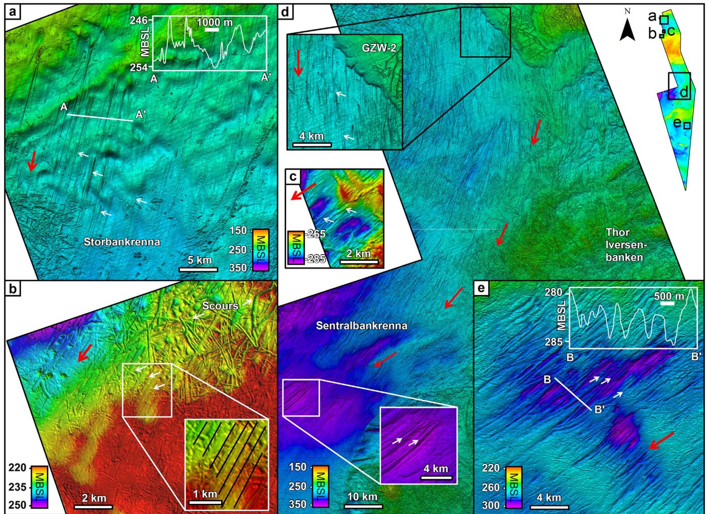
Fig. 4. Examples of mega-scale glacial lineations (MSGSLs) with associated elevation profiles across the survey; a) MSGSLs that cross-cut a ridge in Storbankrenna; b) a continuation of the MSGSLs observed in (a) but heavily disrupted by iceberg scours; c) MSGSLs related to the earliest conditions of ice streaming in Storbankrenna. The MSGSLs have been partially buried by retreat moraines; d) MSGSLs in Sentralbankrenna showing ice flow pathway. The upper inset panel shows the apparent continuation of the MSGSLs beneath the grounding-zone wedge. These MSGSLs have been partially imaged by Bjarnadóttir et al. (2014) in the area of the lower inset; e) MSGSLs in the southern part of the survey to the north of Tiddlybanken. In each panel the white arrows point to individual lineations and the red arrows show the dominant orientation and inferred ice flow pathway. (For interpretation of the references to colour in this figure legend, the reader is referred to the web version of this article.)
