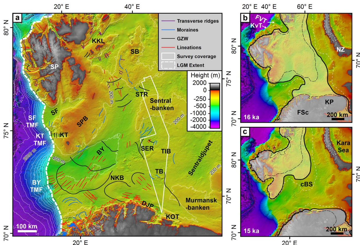
Fig. 1. a) Barents Sea regional bathymetry and hinterland topography from the International Bathymetric Chart of the Arctic Ocean v.3.0 (IBCAO) (Jakobsson et al., 2012b). Contours are every 200 m and the seafloor geomorphology is collated from a number of studies (Ottesen et al., 2008b; Winsborrow et al., 2010; Bjarnadóttir et al., 2014; Jakobsson et al., 2014). The data used in this study is shown with the white outline; b-c) time-slice reconstructions of the Barents Sea Ice Sheet at 16 ka and 15 ka from Hughes et al. (2016). It is important to note that the spatio-temporal evolution of the margin here is uncertain and the white and black dashed lines are the maximum and minimum reconstructions, respectively. The semi-transparent polygons with the thick black outline represents the 'most-credible' reconstruction from Hughes et al. (2016) and it is these reconstructions we use to aid our own. Key place names and abbreviations are as follows: Bjørnøyrenna (BY), central Barents Sea (cBS), Djuprenna (DJP), Fennoscandia (FSc), Franz Victoria Trough (FVT), Grounding-zone Wedge (GZW), Kola Peninsula (KP), Kong Karls Lands (KKL), Kola Trough (KOT), Kveithola Trough (KT), Kvitøya Trough (KvT), Nordkappbanken (NKB), Novaya Zemlya (NZ), Sentralbanken (SER), Spitsbergen (SP), Spitsbergenbanken (SPB), Storbanken (SB), Storbankrenna (STR), Storfjordrenna (SF), Thor Iversen-banken (TIB), Tiddlybanken (TB), and Trough Mouth Fan (TMF). Map projection here and in all subsequent figures is ED50 UTM Zone 33.
