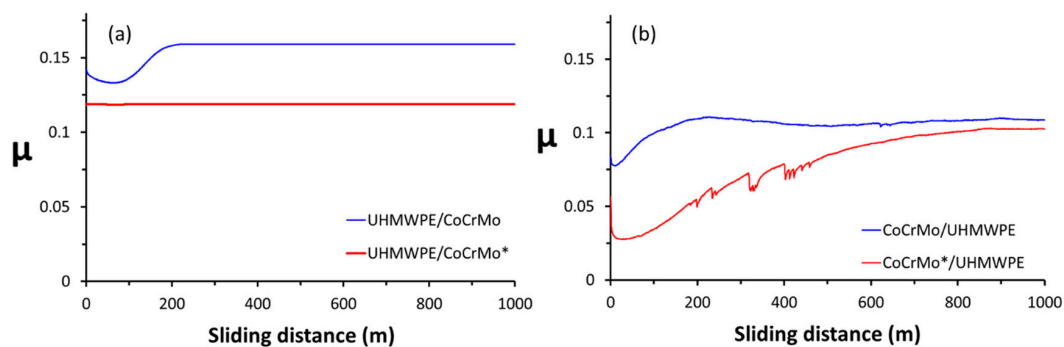
Figure 3. The \mu vs. distance for (a) ultrahigh molecular weight polyethylene (UHMWPE)/CoCrMo and UHMWPE/CoCrMo* (b) CoCrMo/UHMWPE and CoCrMo*/UHMWPE in FBS. The load was 10 N, and the sliding speed was 50 mm/s.
