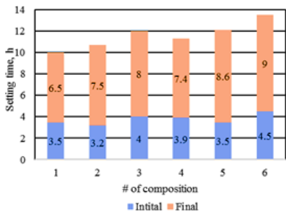
Fig. 6. Setting time of low-clinker BFSC
