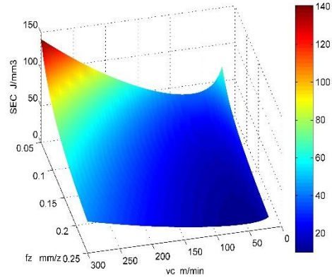
Fig.7. SEC_{total} changes with respect to cutting velocity and feed rate per tooth ( a_p=2.5\text{mm} )
