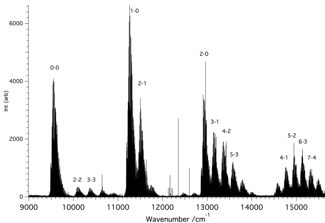
Figure 1. Overview of the Fourier transform emission spectrum of the first positive system of N 2 , identifying the strongest bands in the B 3 Π g – A 3 Σ u + system. Some N I atomic lines also appear. Intensities have been corrected for instrumental response.
